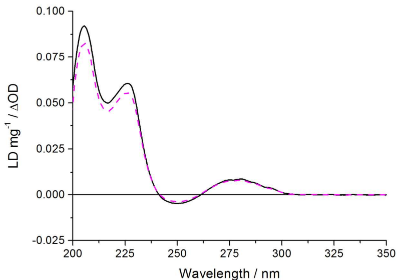
Figure 3. A comparison of the alignment of wtM13 (solid black line) and M13-R-For (pink dashed line) in shear flow using LD spectroscopy. 50 mM potassium phosphate buffer pH 8, 150 mM NaCl. Couette flow 3000 rpm
