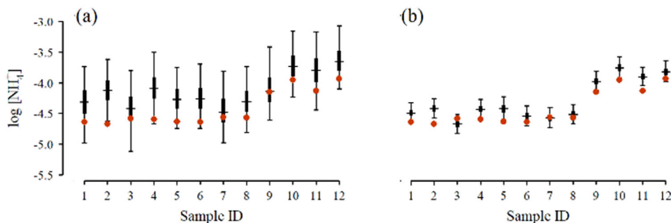
FIGURE 4 [\text{NH}_4^+] in soils samples obtained by direct potentiometry (A) and the standard addition method (B) using an array of four ISEs; [\text{NH}_4^+] measured by FIA are overlaid (red circles). Error bars indicate 95% credible intervals; middle 50% indicated by thick bars; wide dashes represent Bayesian point estimates using the posterior median
