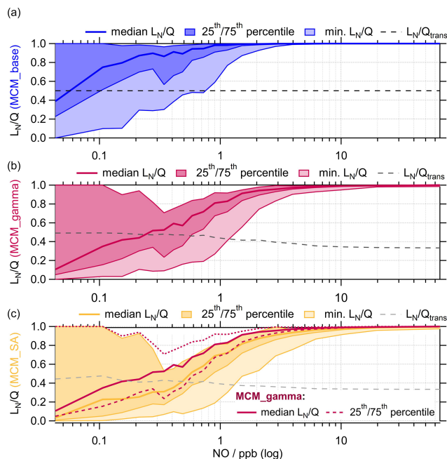
Figure 10. \frac{L_N}{Q} for MCM_base (blue, a), MCM_gamma (pink, b) and MCM_SA (yellow, c) binned against the log of measured NO mixing ratio for the entire summer AIRPRO campaign. \frac{L_N}{Q_{\text{trans}}} for MCM_base (black dashed line) taken as 0.5 for the entire range of NO mixing ratios. \frac{L_N}{Q_{\text{trans}}} for MCM_gamma (dark-grey dashed line) and MCM_SA (light-grey dashed line) calculated using Eq. (10). The 25th and 75th percentiles and minimum \frac{L_N}{Q} are plotted to show the full spread of data for each model scenario.
