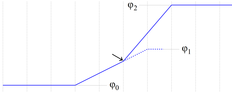
Figure 4: A formant commences a transition from \varphi_0 to its successor \varphi_1 but changes direction towards \varphi_2 before reaching it. We view \varphi_1 as having a dwell of length -1 .
