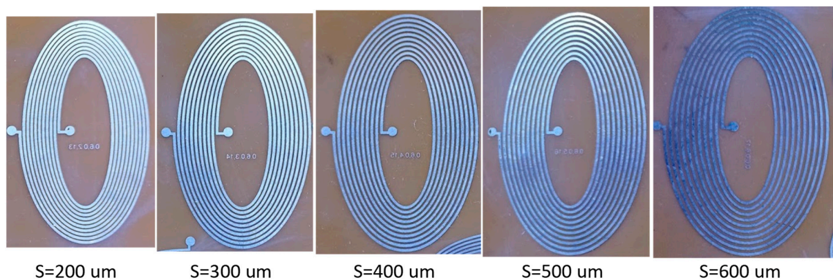
Figure 7. Elliptical planar inductors with a width of 600 μm and varying separation ( S ) while major-to-minor ratio ( R ) = 3 and number of turns ( N ) = 10 were kept constant.
