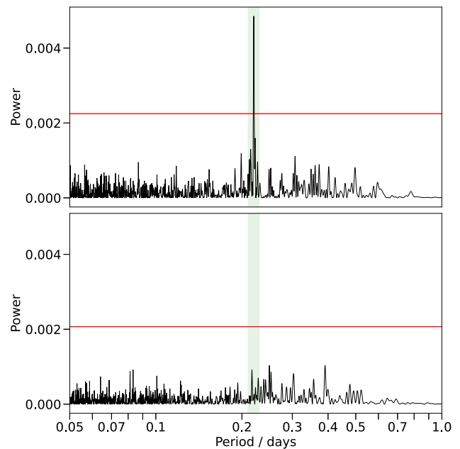
Figure 6. GLS periodogram of the TESS residuals from a global photometric fit using a GP with a Matérn-3/2 kernel to jointly model TESS sector 4 and sector 31. Upper: GLS periodogram of sector 4 residuals. Lower: GLS periodogram of sector 31 residuals. The horizontal red line is the 1 percent false alarm probability level in each case. The significant peak at 0.22004 d in the sector 4 residuals (highlighted in green) is not present in the sector 31 residuals.
