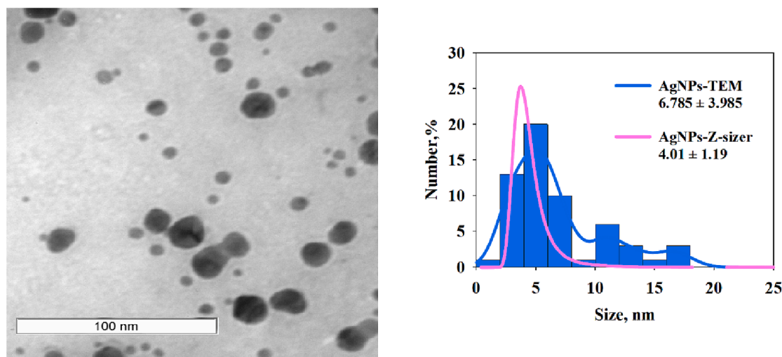
Fig. 7. AgNPs size distribution from TEM and zeta-sizer. AgNPs at 2 \times 10^{-5} dm 3 /min, pH 12, TC 1.91 mM, CR 33.3 dm -1 and ST 0 °C.
