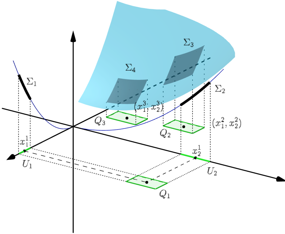
Figure 5. Unveiling the geometric features of the problem when d = 2 . The cubes we find from Theorem 13.10 are weakly transversal, which gives us access to our earlier results.
