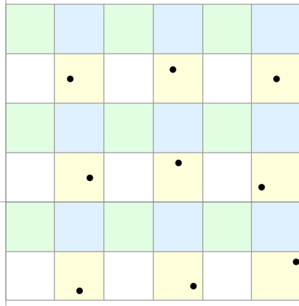
Figure 2. The points \{(x_{2n}, t_{2m})\}_{n,m} .
