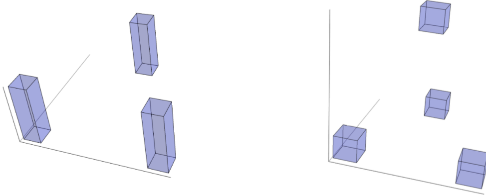
Figure 6. Cases k = 3 and k = 4 when d = 3
