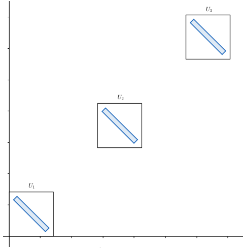
Figure 8. H_j^\delta is supported on U_j .
