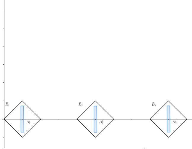
Figure 7. The function h_j^\delta .
