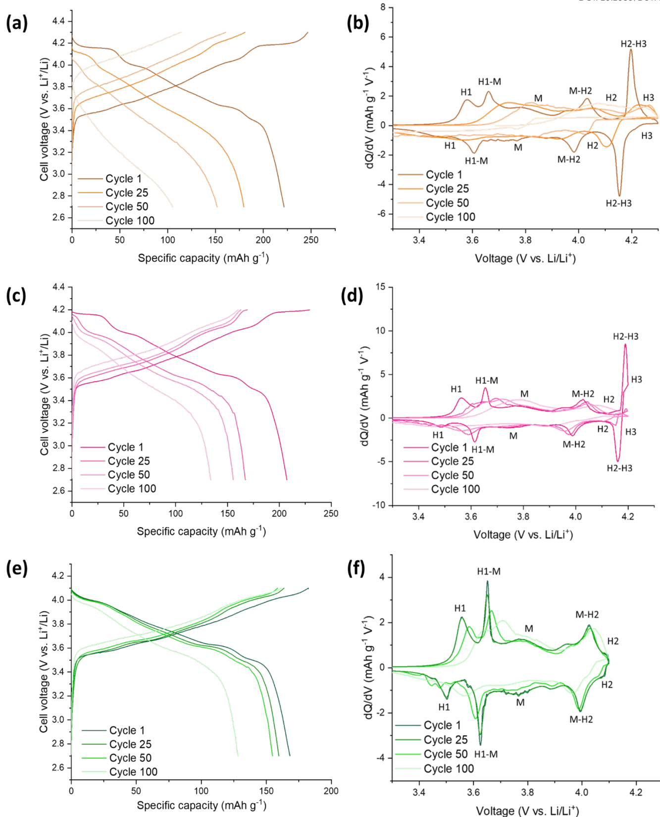
Figure 5- Electrochemical performance during galvanostatic charge and discharge of C-LNO/ Li half cells at 10 mA g -1 : (a) between 2.7 - 4.3 V (b) corresponding differential capacity (dQ/dV) plot with phases (c) between 2.7 - 4.2 V (d) corresponding differential capacity (dQ/dV) plot with phases (e) between 2.7 - 4.1 V (f) corresponding differential capacity (dQ/dV) plot with phases.
