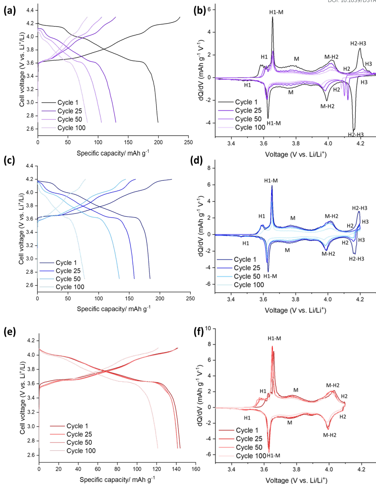
Figure 3- Electrochemical performance during galvanostatic charge and discharge of SS-LNO/ Li half cells at 10 mA g -1 : (a) between 2.7 - 4.3 V (b) corresponding differential capacity (dQ/dV) plot with phases (c) between 2.7 - 4.2 V (d) corresponding differential capacity (dQ/dV) plot with phases (e) between 2.7 - 4.1 V (f) corresponding differential capacity (dQ/dV) plot with phases.
