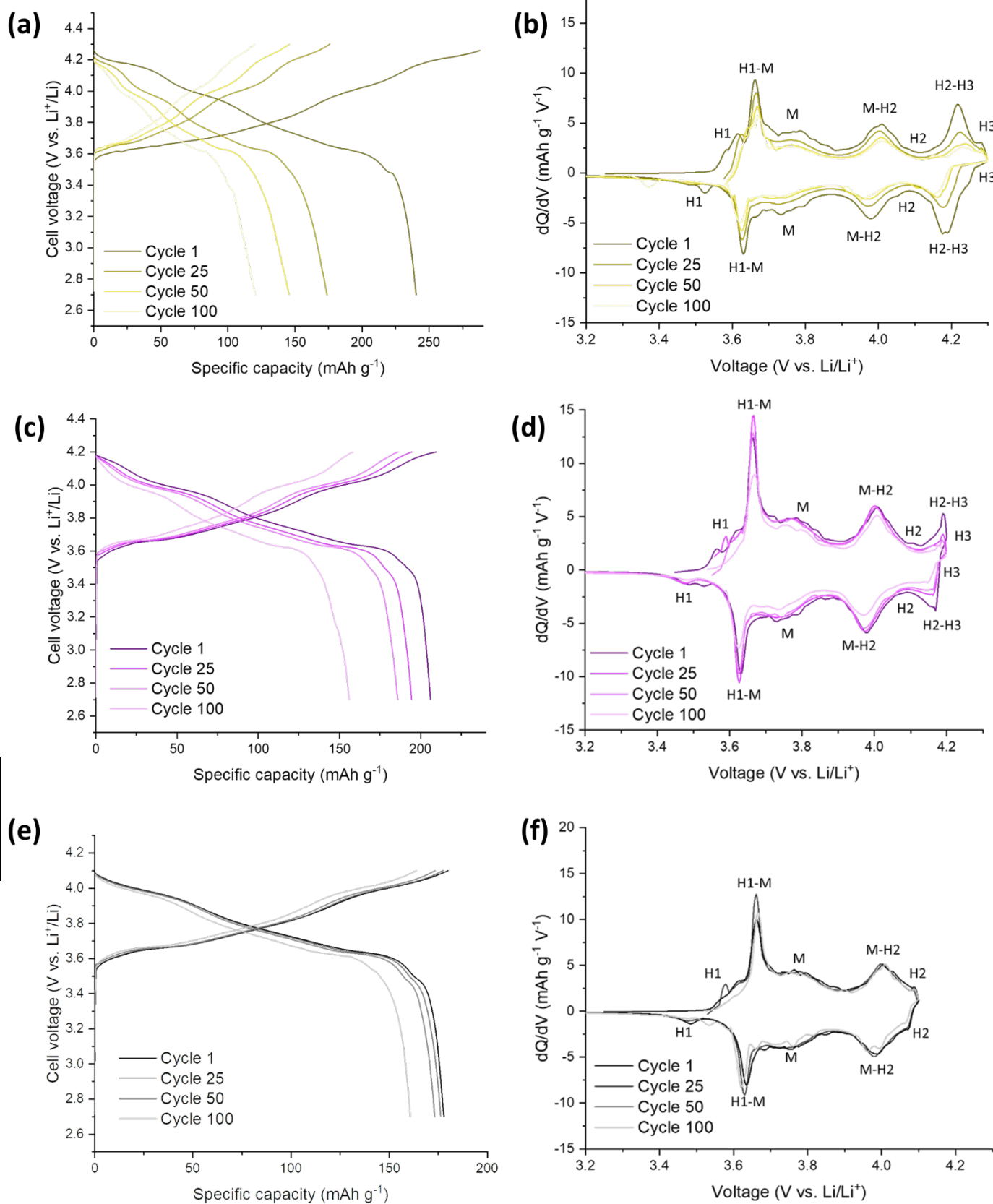
Figure 6- Electrochemical performance during galvanostatic charge and discharge of Mo-LNO/ Li half cells at 10 \text{ mA g}^{-1} : (a) between 2.7 - 4.3 V (b) corresponding differential capacity ( dQ/dV ) plot with phases (c) between 2.7 - 4.2 V (d) corresponding differential capacity ( dQ/dV ) plot with phases (e) between 2.7 - 4.1 V (f) corresponding differential capacity ( dQ/dV ) plot with phases.
