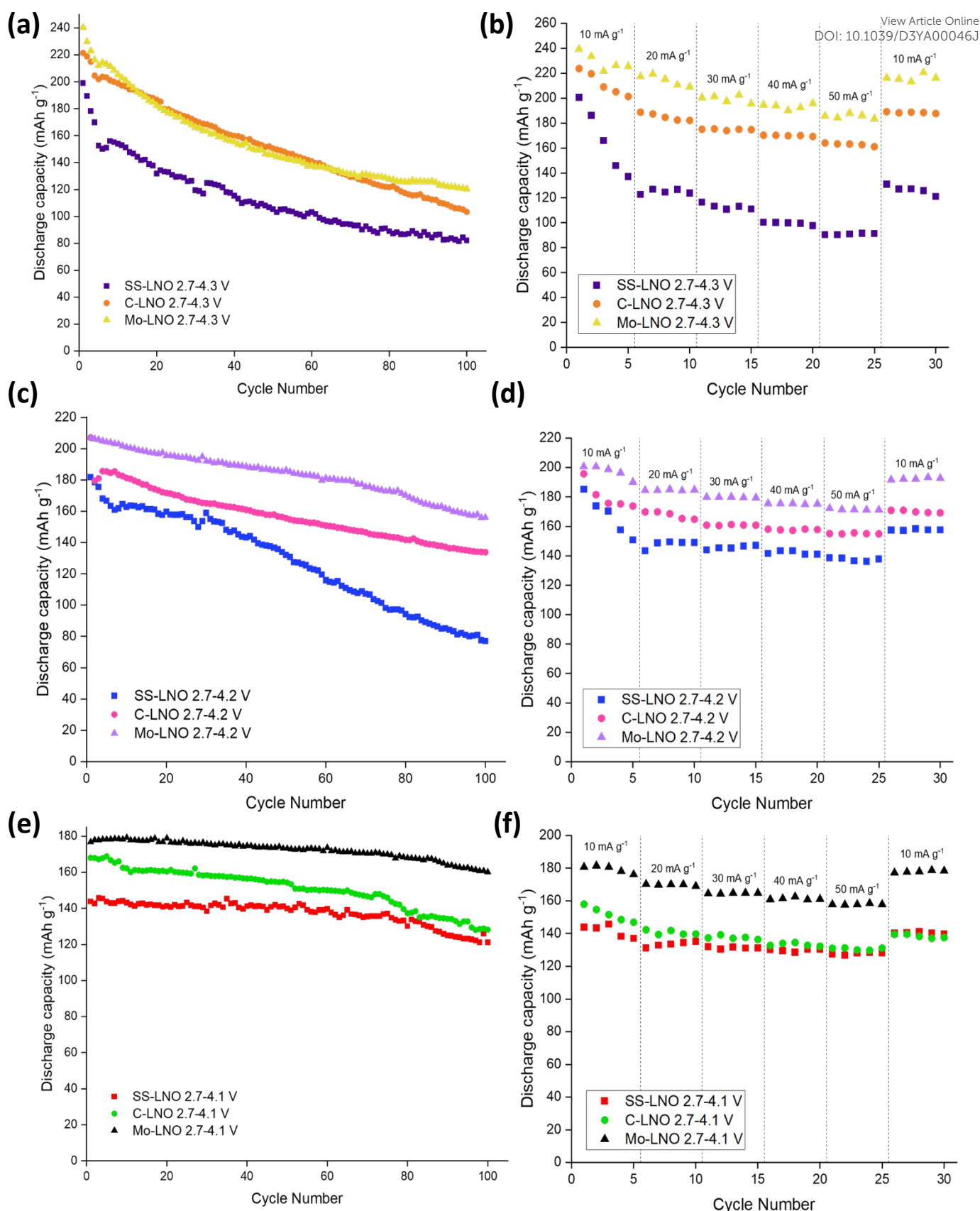
Figure 7- Comparison of SS-LNO, C-LNO and Mo-LNO over 100 cycles at (a) 2.7 - 4.3 V, (c) 2.7 - 4.2 V and (e) 2.7 - 4.1 V. Rate tests also shown between (b) 2.7 - 4.3 V, (d) 2.7 - 4.2 V and (f) 2.7 - 4.1 V for SS-LNO, C-LNO and Mo-LNO.
