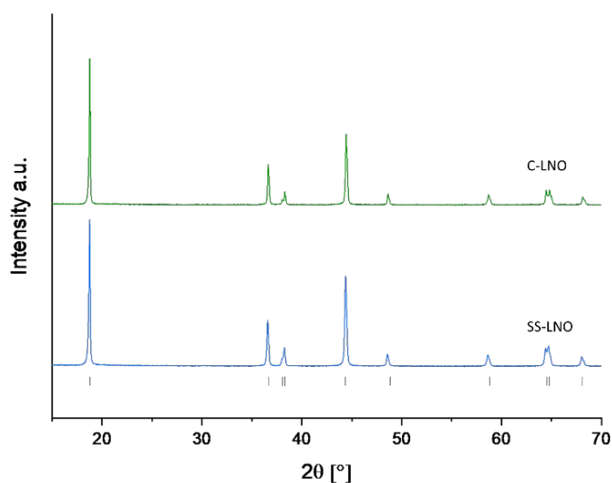
Figure 2-XRD pattern of SS-LNO synthesised at 700 °C for 12 hours in O 2 (blue), and C-LNO synthesised at 800 °C for 1 hour in O 2 (green)
