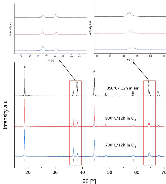
Figure 1-XRD patterns for SS-LNO synthesised at different temperatures and different atmospheres. Caption for each pattern outlines: sintering temperature, sintering time and atmosphere used. Boxed Regions shown zoomed images of peak splitting.
