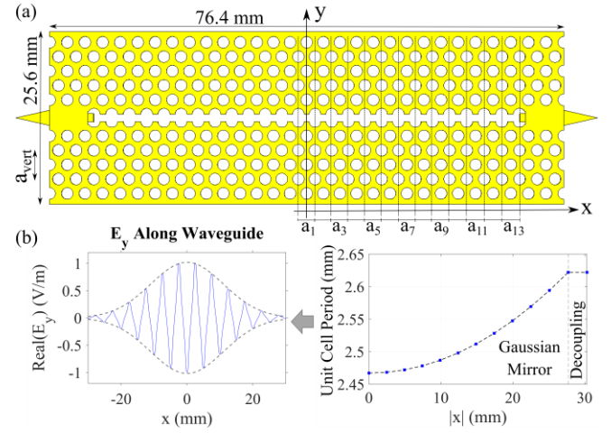
Fig. 1. (a) The EBG resonator with its dimensions and variable periodicity ( a_n ) along the x -axis. (b) The Gaussian envelope of the resonant mode achieved by linearly increasing the reflection from the center to the outer unit cells.
