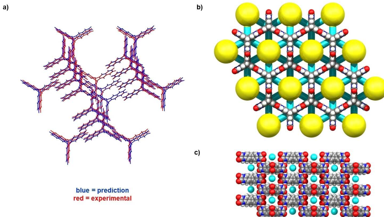
Figure 2. a) Crystal packing similarity search performed in Mercury [26] between the CSP structure, \text{TH5-A} (blue) [27] and \text{TH5}\alpha\text{-acetone} (red). The search yielded an RMSD of 0.399 Å for a 20-molecule comparison. b, c) Crystal packing in \text{TH5}\alpha\text{-Acetone} showing hexagonal pores (yellow) running along the crystallographic c -axis and interconnecting channels (turquoise) running along the crystallographic a and b -axes. Solvent molecules are omitted for clarity.
