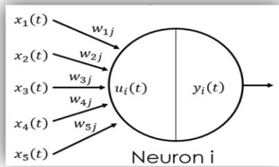
Figure 1. Artificial neuron
