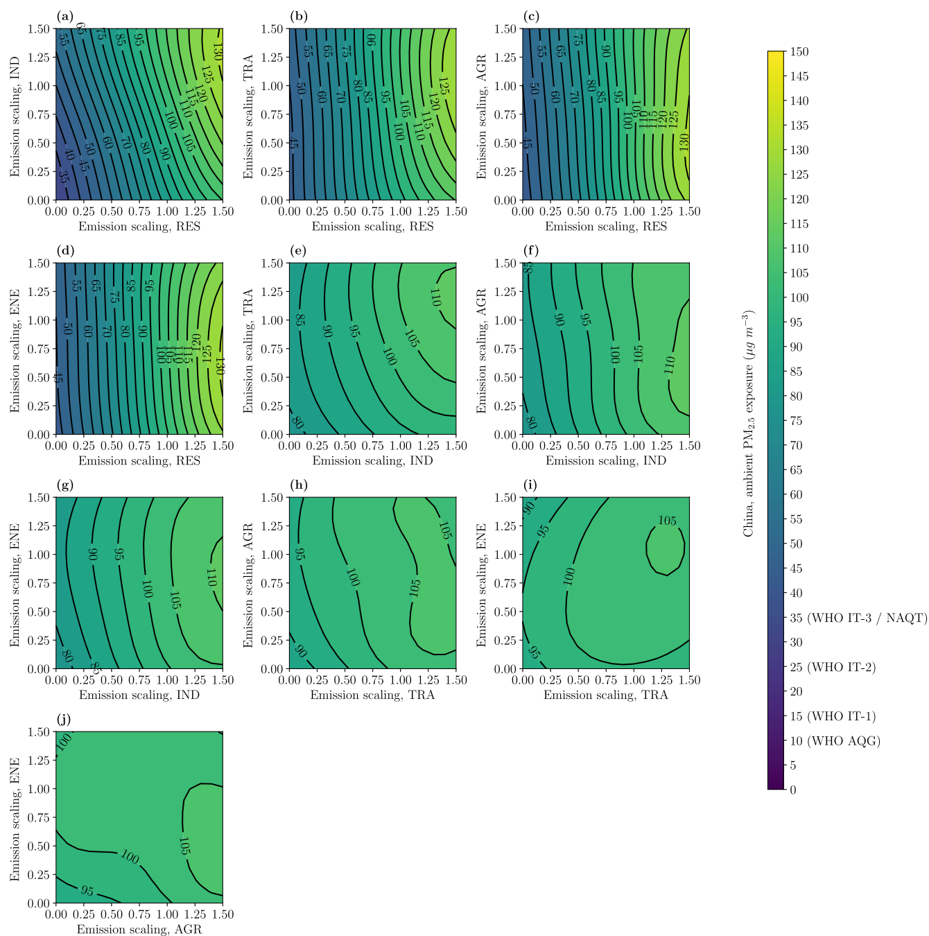
Figure 5. The combined impact of variations in two emission sectors on ambient fine particulate matter ( PM_{2.5} ) exposure for China from (a) residential (RES) and industry (IND), (b) RES and land transport (TRA), (c) RES and agriculture (AGR), (d) RES and power generation (ENE), (e) IND and TRA, (f) IND and AGR, (g) IND and ENE, (h) TRA and AGR, (i) TRA and ENE, and (j) AGR and ENE emissions. Air quality targets shown for the World Health Organization's (WHO) Air Quality Guideline (AQG), Interim Target 1 (IT-1), Interim Target 2 (IT-2), Interim Target 3 (IT-3), and China's National Air Quality Target (NAQT).
