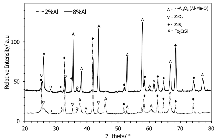
Figure 11. X-ray diffraction pattern of the ablated front side of the samples.
