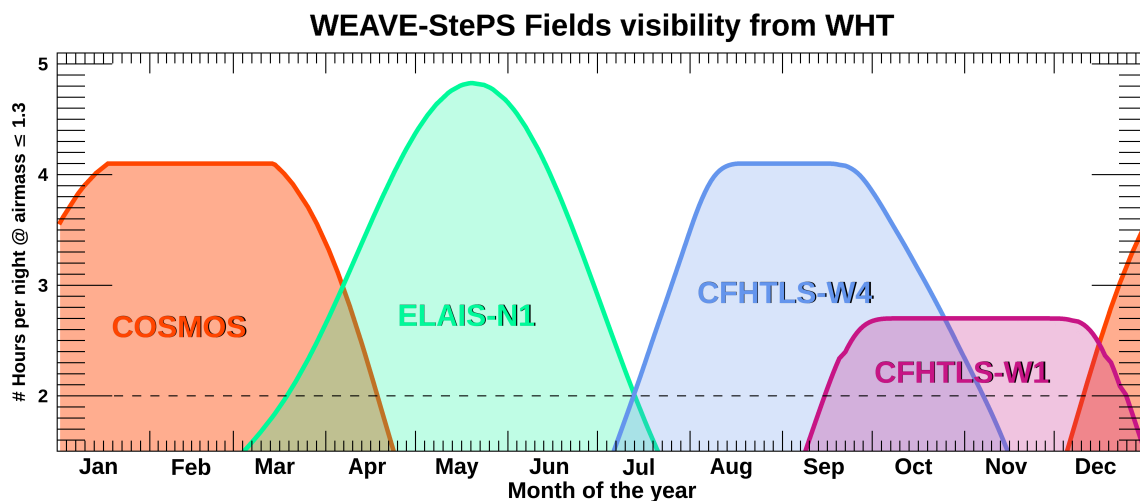
Fig. 6. Number of hours per night at an airmass below 1.3 for each of the planned WEAVE-StePS fields (as labelled) throughout the year.
