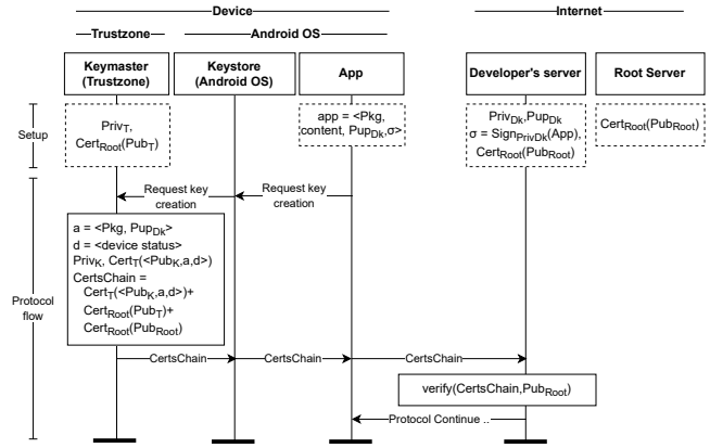
Figure 2: Android Key Attestation protocol based on [8]
