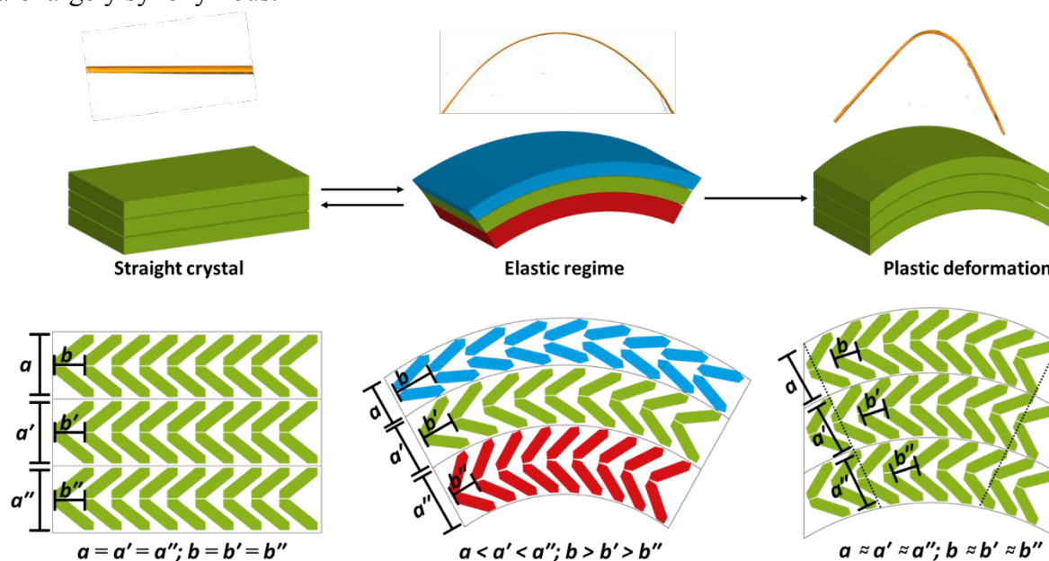
Fig. 6 | Schematic mechanisms for mechanical flexibility in DMP. Elastic bending regime. As the crystal bends, a region of high pressure (red) is generated at the concave face, with a region of low pressure (blue) generated at the convex face. The former leads to shortening of the crystal along the bending axis (010), and elongation along the perpendicular axis. Simultaneously, the low-pressure region at the convex face leads to growth of the (010) axis, and shortening of the other crystal direction. Plastic bending regime. Once the accumulated strain overcomes the slip plane energy (shown as curved horizontal grey lines), delamination along this slip plane occurs until balance between compression and slip plane energies is restored (hence residual elasticity in plastic regime).
