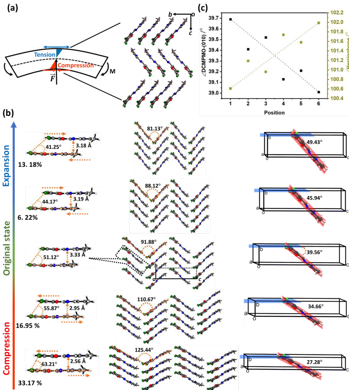
Fig. 4 | Bending model for elastically flexible single crystals. (a) Ideal bending model for a beam, in which the impinging force, \vec{F} , causes a bending moment, M , driving compression at the concave face of the beam and expansion at the convex face of the beam. A neutral axis (dashed line) passes through the centre of the crystal, in which no deformation occurs. (b) The angle between DMP molecules and the (010) plane, and the angle of the herringbone layer, as obtained from experimental \mu -focus XRD data. (c) Ab initio (PBE-D2) investigation of the anisotropic compression and expansion of DMP single crystals along the crystallographic b -axis. We note that extension and compression have been exaggerated to facilitate visualisation of the structural response.
