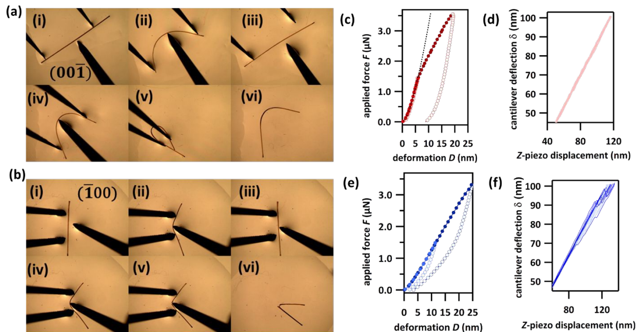
Fig. 2 | Mechanical properties of DMP single crystals. (a-b) Optical microscope photographs of three-point bending experiments of single crystals of DMP over the (a) (00\bar{1}) , and (b) (\bar{1}00) crystallographic faces. Note that bending over the (00\bar{1}) face is fully reversible below a certain load (i-iii). With increasing load, it exhibits plastic deformation (iv-vi). (c-f) Atomic force microscopy (AFM) force-deformation curves (FDC) for the (c) (00\bar{1}) and (e) (\bar{1}00) crystallographic faces, alongside the partial corresponding raw deflection-displacement curves for (d) (00\bar{1}) and (f) (\bar{1}00) . AFM FDCs were measured using a 150 \pm 10 nm radius; the AFM tip was made from electron beam deposited high density carbon. A fit to Hertz theory estimates the Young's modulus of DMP over the (00\bar{1}) face (see black dashed line in (c)) to be 5.7 GPa (Poisson ratio \nu = 0.3 ). Averaged curves from at least 30 curves are presented. Filled markers in (c) and (e) correspond to the approach part of the measurements, empty circles to the retract part. The experiments with applied maximal forces F < 1.5 \mu\text{N} are presented in light red (c) and light blue (e), experiments with applied maximal forces F > 1.5 \mu\text{N} are presented in dark red (c) and dark blue (e).
