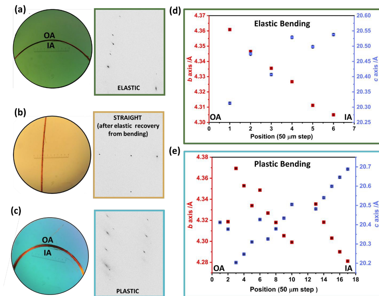
Fig. 3 | Synchrotron-based \mu -focus X-ray diffraction of mechanically bent single crystals of DMP. (a) Photograph of elastically bent single crystal alongside an excerpt of the Bragg scattering obtained from within the bent region of the crystal. (b) Photograph of the elastically bent crystal after release of one end, alongside the associated Bragg scattering
