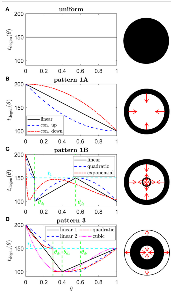
FIGURE 5 | Target cone degeneration profiles. Panels (left) show cone degeneration profiles, t_{\text{degen}}(\theta) , qualitatively replicating typical spatio-temporal patterns of visual field loss in RP: (A) Uniform, (B) Pattern 1A, (C) Pattern 1B and (D) Pattern 3. Visual field loss patterns directly correspond to cone degeneration patterns in these radially symmetric cases. We seek to replicate these patterns by finding appropriate \phi_{\text{rim}}(\theta) and f_{\text{crit,rim}}(\theta) profiles in Figures 6–9 . Diagrams on the right show the corresponding 2D patterns of visual field loss — white regions: preserved vision, black regions: scotomas (blind spots), and red arrows: direction of scotoma propagation. Parameters: t_0 = 100 (~ 11.0 years), t_1 = 150 (~ 16.6 years), t_2 = 200 ~ 22.1 years, \theta_{d_1} = 0.1 (~ 7.6 degrees), \theta_{d_2} = 0.55 (~ 41.9 degrees), \theta_{d_3} = 0.3 (~ 22.9 degrees), \theta_{d_4} = 0.4 (~ 30.5 degrees) and \theta_{d_5} = 0.6 (~ 45.7 degrees). Cone degeneration profile formulas and parameters are given in Table 3 . Remaining parameter values as in Table 2 .
