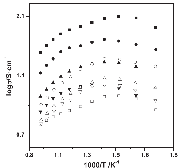
Fig. 7. Plot of \log \sigma vs 1000/T for SrFeO 3-δ (■), SrFe 0.95 Ge 0.05 O 3-δ (●), SrFe 0.90 Ge 0.10 O 3-δ (▲), SrFe 0.85 Ge 0.15 O 3-δ (▼), Sr 0.75 Ca 0.25 FeO 3-δ (□), Sr 0.75 Ca 0.25 Fe 0.95 Ge 0.05 O 3-δ (○), Sr 0.75 Ca 0.25 Fe 0.90 Ge 0.10 O 3-δ (△) and Sr 0.75 Ca 0.25 Fe 0.85 Ge 0.15 O 3-δ (▽).
