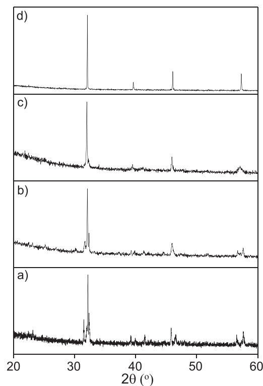
Fig. 3. X-ray diffraction patterns for (a) \text{SrFeO}_{3-\delta} , (b) \text{SrFe}_{0.95}\text{Ge}_{0.05}\text{O}_{3-\delta} , (c) \text{SrFe}_{0.90}\text{Ge}_{0.10}\text{O}_{3-\delta} and (d) \text{SrFe}_{0.85}\text{Ge}_{0.15}\text{O}_{3-\delta} , annealed at 800 °C for 24 h in 5% \text{H}_2 –95% \text{N}_2 , showing a stabilisation of the cubic phase under these conditions on increasing the Ge content.
