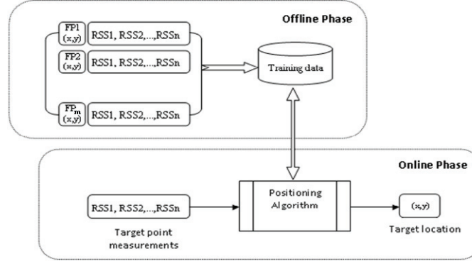
Fig 2 fingerprint block diagram
