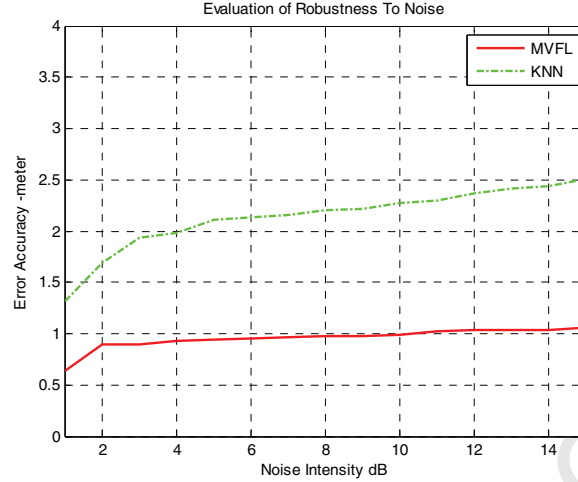
Fig 11 MVFL vs kNN robustness against noise
