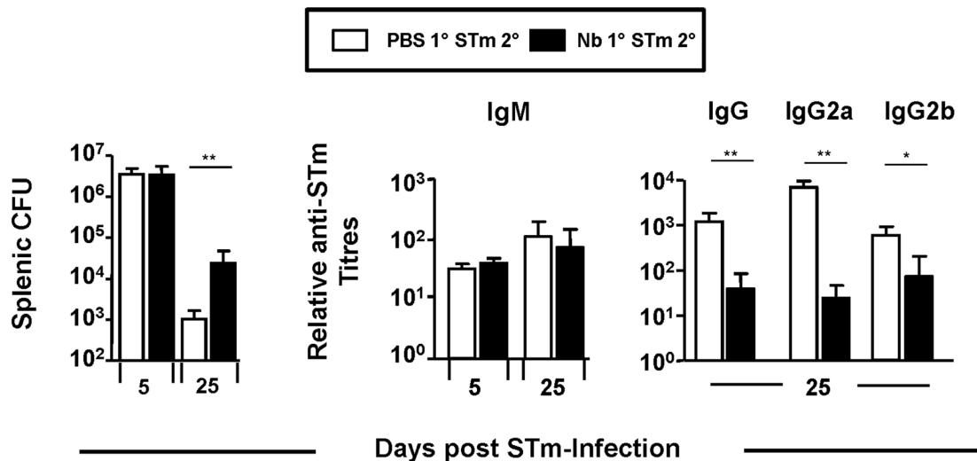
Figure 6. Prior Infection with Nb alters the control of STm and production of anti-STm IgG. WT mice were infected with 500 L3 Nb larvae and at day 16 mice were challenged with 5 \times 10^5 STm alongside naïve control mice. Splenic bacterial numbers were assessed at days 5 and 25 post-STm infection. Serum anti-STm IgM, IgG, IgG2a and IgG2b antibody titres were assessed by ELISA against a total outer membrane preparation of STm. Infections with STm and Nb were administered intraperitoneally and subcutaneously respectively. Groups contained 4–6 mice. (*P<0.05 and **P<0.005). doi:10.1371/journal.pntd.0003341.g006
