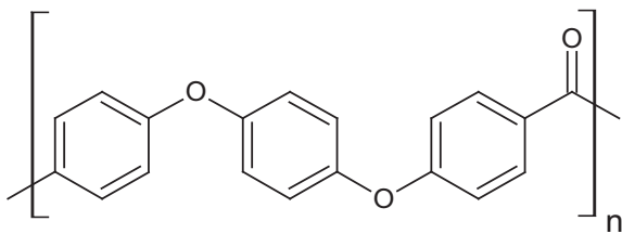
Fig. 1. Structure of poly(oxy-1,4-phenyleneoxy-1,4-phenylenelecarbonyl-1,4-phenylene) PEEK.
