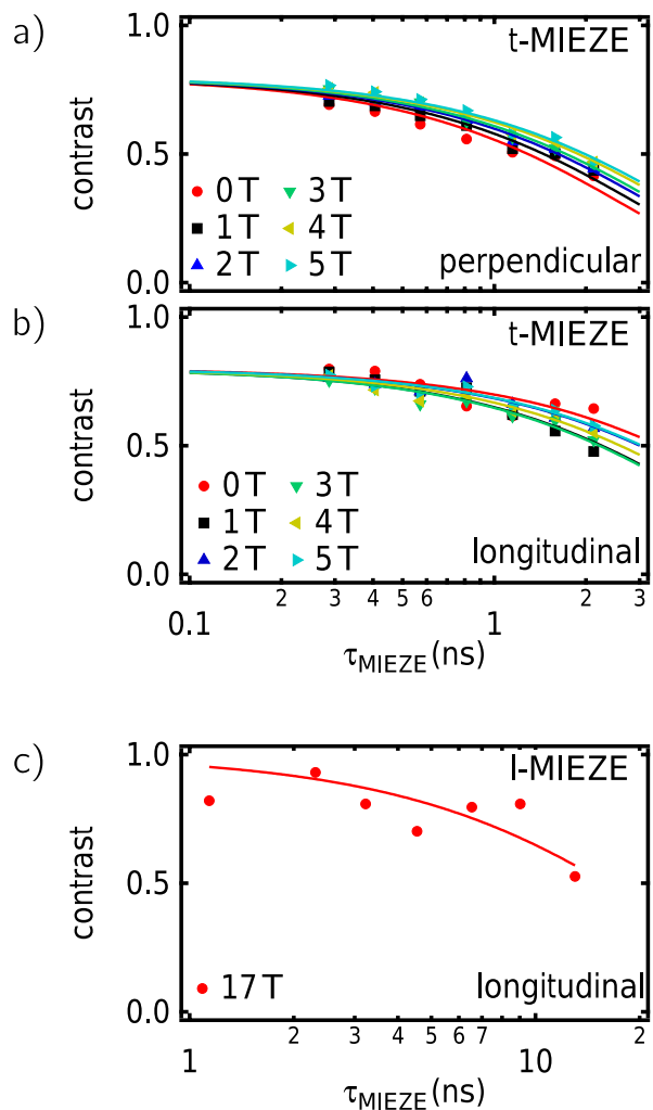
Figure 4. MIEZE resolution with magnetic field at the sample. a) Typical data as recorded with a 5 T SANS magnet, where the field was applied perpendicular to the neutron beam. b) same as for a) for magnetic field applied longitudinal to the neutron beam. c) Typical data as recorded at 17 T applied longitudinal to the neutron beam using the Birmingham SANS magnet [19].
