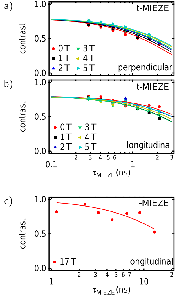
Figure 4. MIEZE resolution with magnetic field at the sample. a) Typical data as recorded with a 5 T SANS magnet, where the field was applied perpendicular to the neutron beam. b) same as for a) for magnetic field applied longitudinal to the neutron beam. c) Typical data as recorded at 17 T applied longitudinal to the neutron beam using the Birmingham SANS magnet [19].
