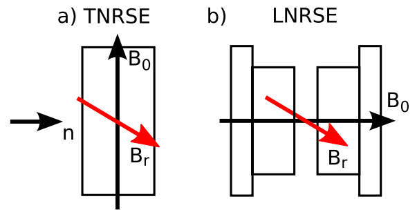
Figure 2. Schematic drawing of a TNRSE coil a) and LNRSE coil b). The neutron beam ( n ) traverses the coils from the left side as indicated by the arrow.
