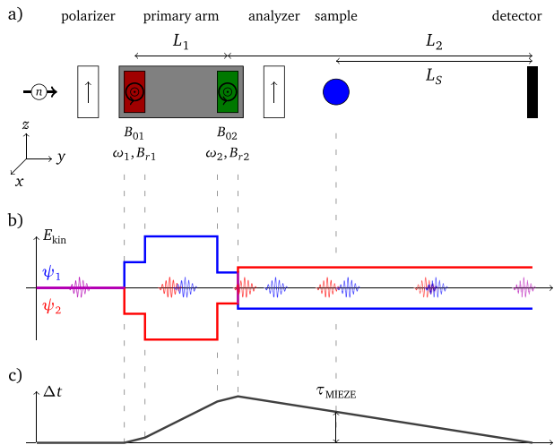
Figure 1. Principles underlying the MIEZE technique. a) Schematic depiction of a MIEZE-1 setup. b) Kinetic energy of the neutron as function of flight path. c) Temporal separation of the neutron spin wave function as function of the flight path. The MIEZE time \tau_{\text{MIEZE}} is defined by the separation at the sample position. Figure after [2].
