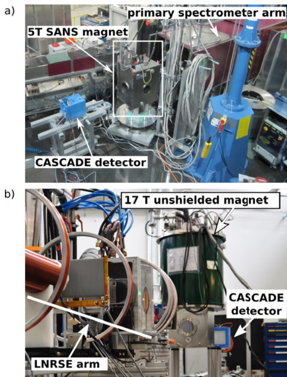
Figure 3. MIEZE and magnetic field setup at RESEDA. a) Transverse MIEZE setup as combined with an actively shielded 5 T SANS magnet from the MLZ sample environment group. b) Longitudinal MIEZE setup as combined with the Birmingham 17 T magnet [19]. This magnet does not offer active stray-field reduction.
