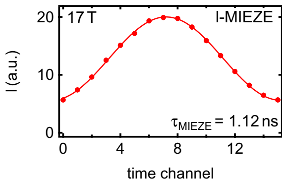
Figure 5. Typical MIEZE echo measured with the I-MIEZE setup. The echo was recorded under an applied field of 17 T at a frequency of \omega_2 = 77 kHz. The solid line is a cosine fit to the data.
