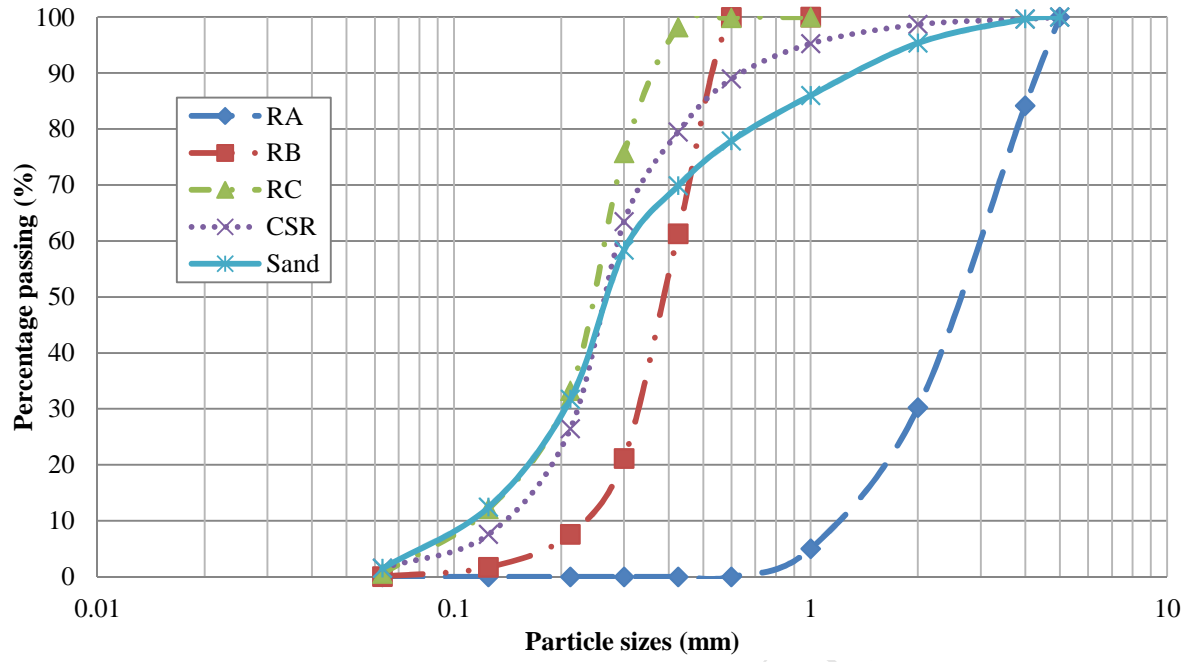
Fig. 1: Grading curves of sand and rubber particles
