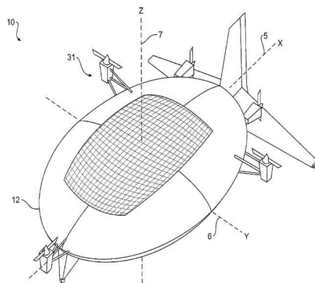
Figure 3. A possible lighter than air platform for solar energy collection, reproduced with permission. 74 Copyright 2014, United States Patent.
