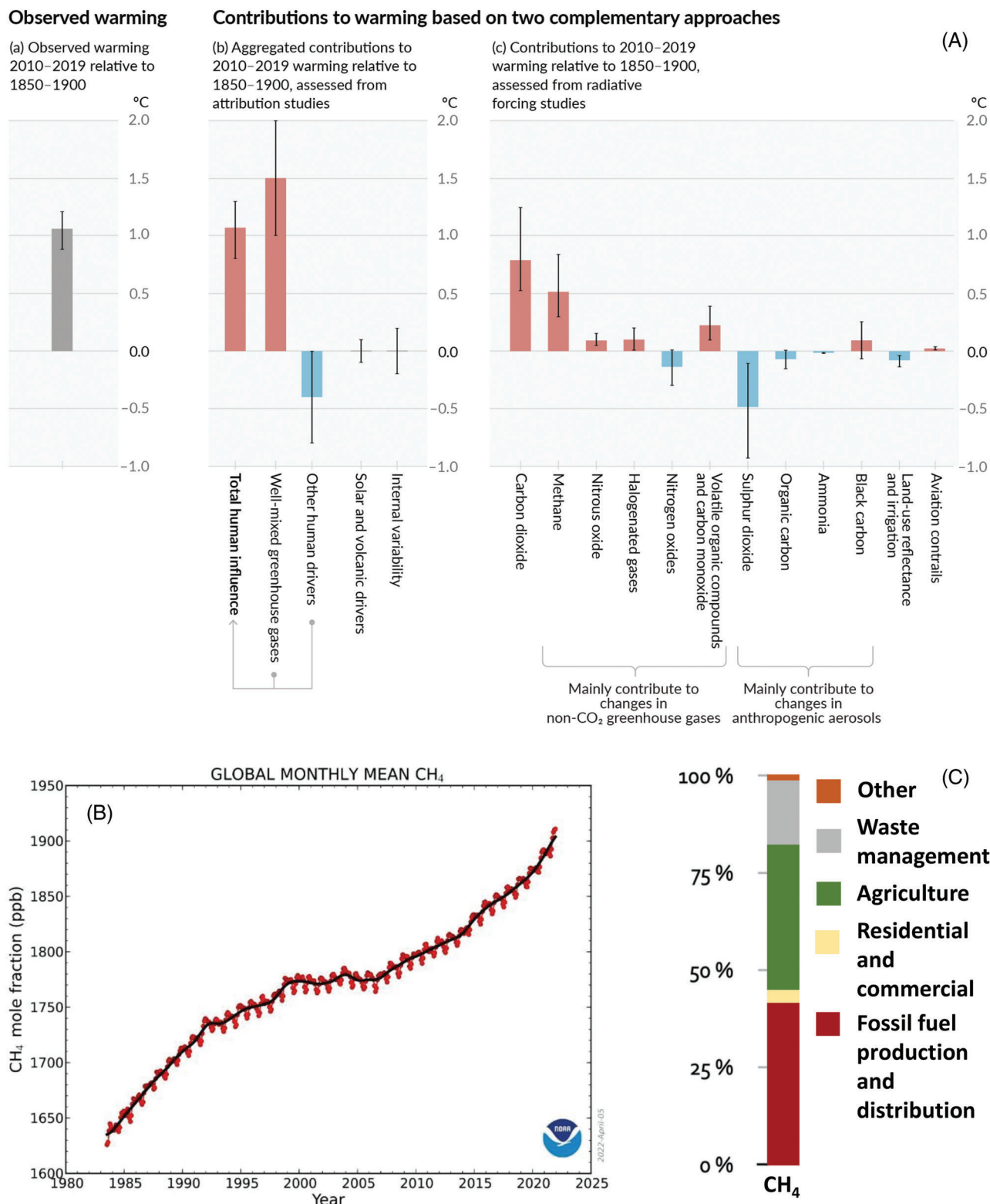
Figure 1. A) Assessed contributions of various warming factors to observed warming in 2010–2019 relative to 1850–1900. Reproduced with permission. 2 Copyright 2021, IPCC. (B) Globally-averaged, monthly mean atmospheric CH 4 concentration since 1983. (NOAA Global Monitoring Laboratory). (C) Relative sectoral contributions to the anthropogenic emissions of CH 4 . 2 Copyright 2021, IPCC.
