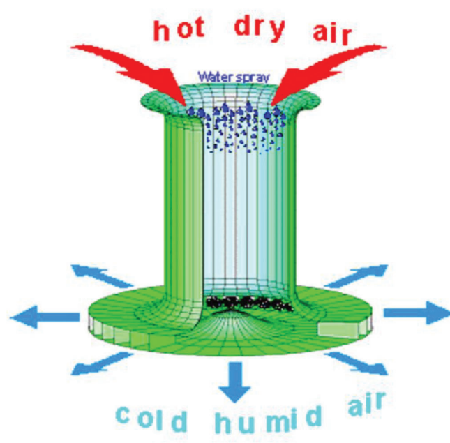
Figure 2. Schematic illustration of the energy tower, Reproduced with permission. 60 Copyright Czisch and Technion - Israel Institute of Technology.
