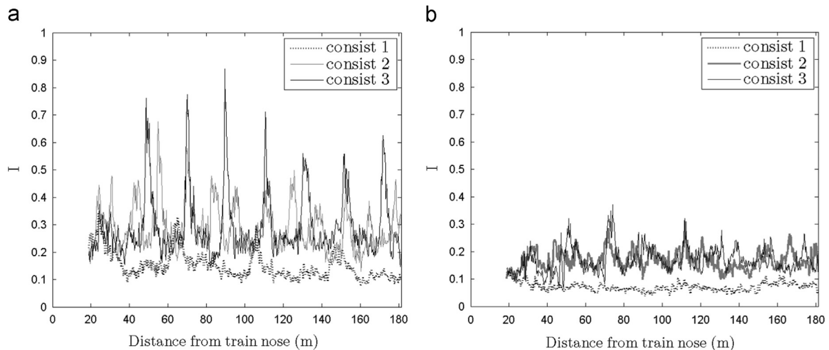
Fig. 13. Turbulence intensities for the 8 wagon train with freight consists 1, 2 and 3. Measurements are made at train side at a height of z=2.25 m at distance y=1.75 m from the centre of track and above the train roof at a height of z=4.5 m and a distance of y=0 m from the centre of track. a) Probe 1 and b) Probe 3.
