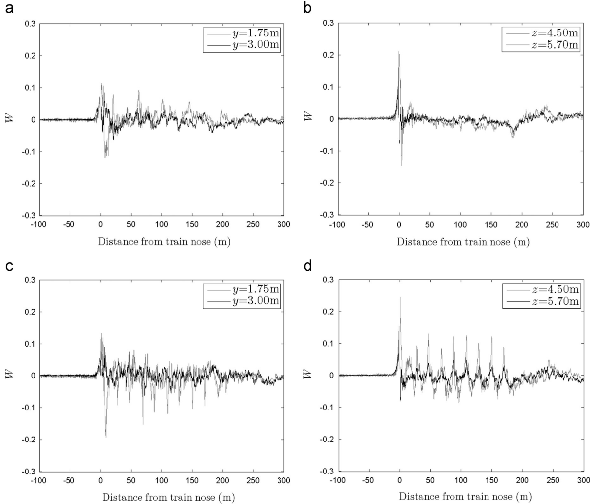
Fig. 12. The normalised ensemble vertical component of velocity W for the 8 wagon train with freight consists 1 and 3. Measurements are made at train side at a height of z=2.25 m at distances y=1.75 m and y=3 m from the centre of track, and above the train roof for heights z=4.5 m and z=5.7 m at a position of 0 m from the centre of track a) Consist 1 probes 1 and 2; b) Consist 1 probes 3 and 4; c) Consist 3 probes 1 and 2 and d) Consist 3 probes 3 and 4.
