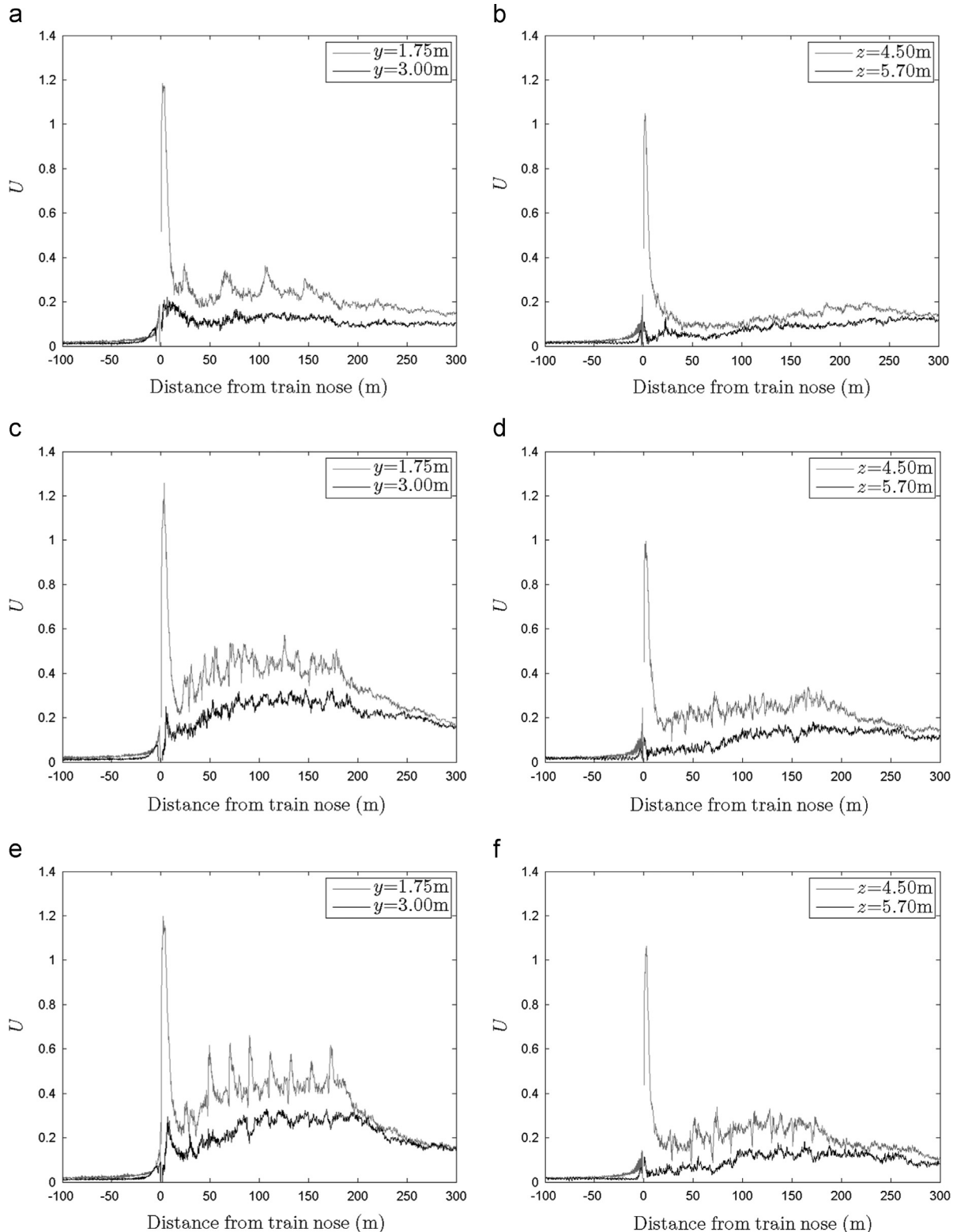
Fig. 8. The normalised ensemble longitudinal component of velocity U for the 8 wagon train. Measurements are made at train side at a height of z=2.25 m at distances y=1.75 m and y=3 m from the centre of track, and above the train roof for heights z=4.5 m and z=5.7 m at a position of 0 m from the centre of track. a) Consist 1 probes 1 and 2; b) Consist 1 probes 3 and 4; c) Consist 2 probes 1 and 2; d) Consist 2 probes 3 and 4; e) Consist 3 probes 1 and 2 and f) Consist 3 probes 3 and 4.
