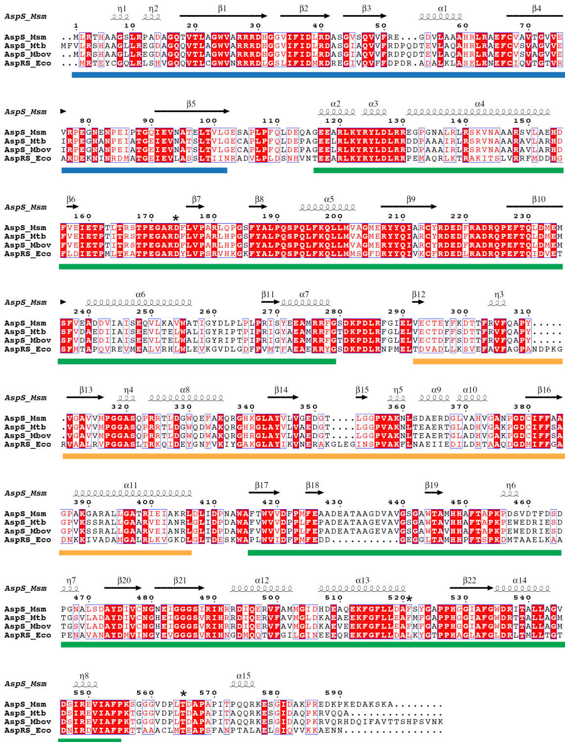
Figure 7. Alignment of the amino acid sequences of AspS of M. smegmatis (Msm), M. tuberculosis (Mtb) and M. bovis (Mbv) with that of E. coli AspRS (Eco). Bars in blue, green and orange indicate the N-terminal, catalytic and insertion domains of AspS, respectively. Asterisks indicate the sites of resistance-conferring mutations. doi:10.1371/journal.pone.0113568.g007
