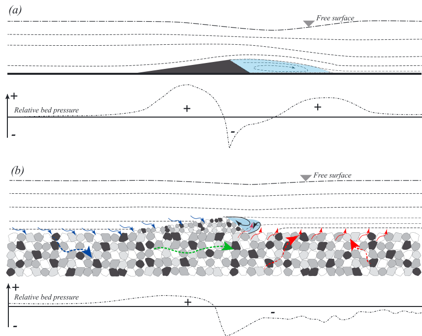
Figure 4. Schematic summary of flow around (a) reference case: impermeable bed form over impermeable smooth bed (IDIB), (b) natural bed form in coarse gravel bed: permeable bed form over permeable bed (PDPB). Streamlines over the bed form are shown, with the region in blue denoting the flow separation zone that is radically different in its shape and downstream extent over the PDPB. Note also the flow through the permeable bed form (dashed-large arrows) and upwelling hyporheic flow jets (small red arrowheads) in the leeside of the PDPB. The schematic bed pressure distribution associated with each bed configuration is shown to illustrate the potentially very different bed pressures associated with each bed.
