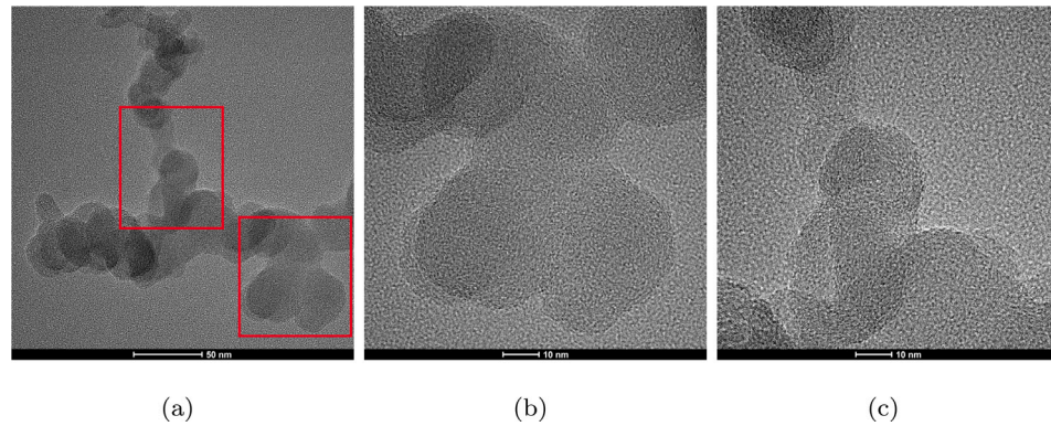
Fig. 3. Soot agglomerate from tests D100M.
