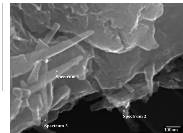
Fig. 11. High magnification SEM images showing oxide whisker formation in the spark plasma sintered NP structure.
