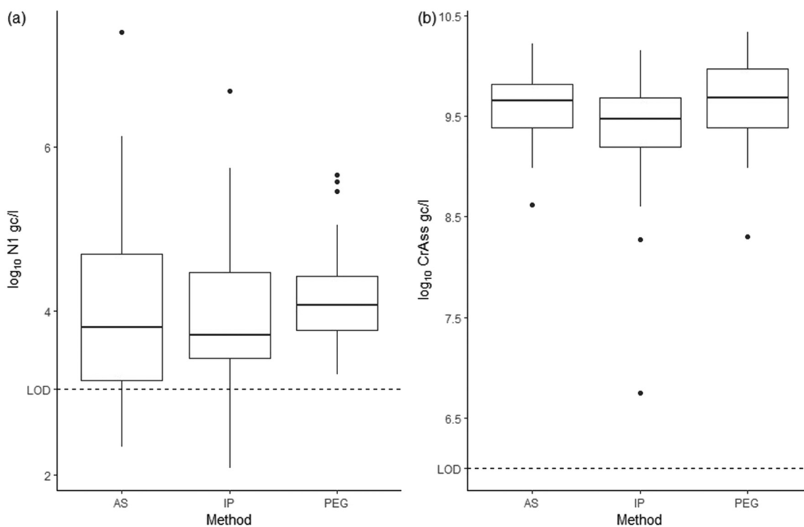
Fig. 1. a) \log_{10} SARS-CoV-2 N1 genome copies per litre (gc/l) among concentration methods ammonium sulphate (AS), polyethylene glycol (PEG) and InnovaPrep (IP). The box depicts percentile ranges from 25, 50, and 75 respectively, the whiskers depict \pm 1.5 \times IQR, and the outliers are indicated by points. b) \log_{10} crAssphage genome copies per litre between concentration methods, the dotted line marks the assay LOD for RT-qPCR.
