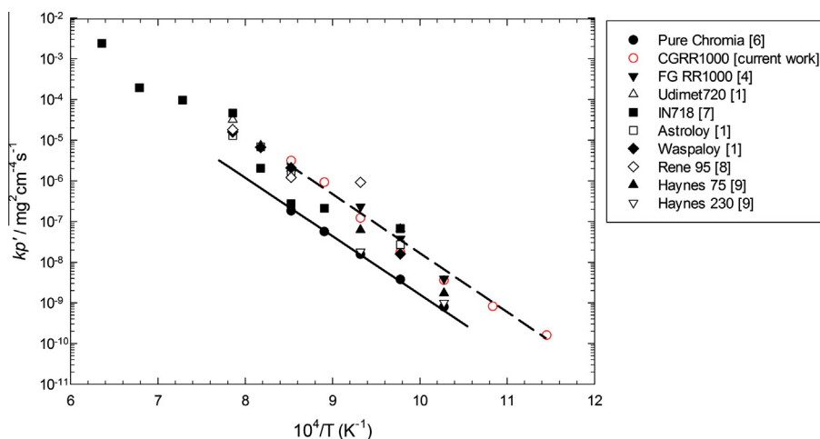
Fig. 3. Arrhenius plot of k'_p values from this study (shown as unfilled circles) and from various superalloys taken from the literature (compiled in [5]). Also shown as the solid line are the expected k'_p values for chromia growth [6] on simpler alloys. All exposures were undertaken in laboratory.
