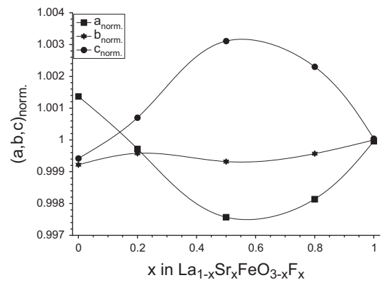
Fig. 6. Dependency of normalized lattice parameters (a,b,c)/\text{norm.} ( k=2^{1/2} for a and c and k=2 for b , taking into account the different lengths of the orthorhombic axes) on the degree of substitution x in \text{La}_{1-x}\text{Sr}_x\text{FeO}_{3-x}\text{F}_x . For x=0 , lattice parameters were determined from XRD data only.
