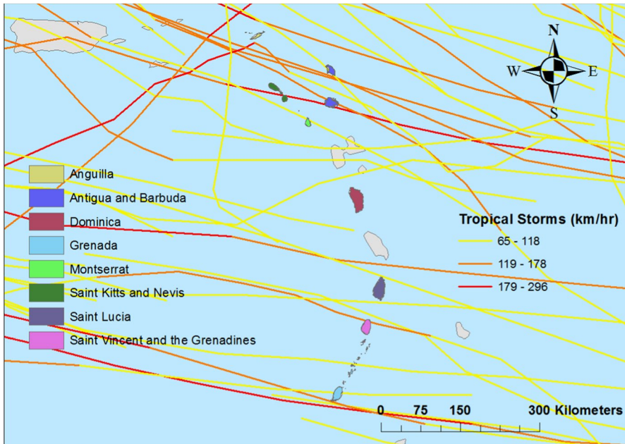
Fig. 1 Eastern Caribbean Island sample and tropical storms (1996–2013)
