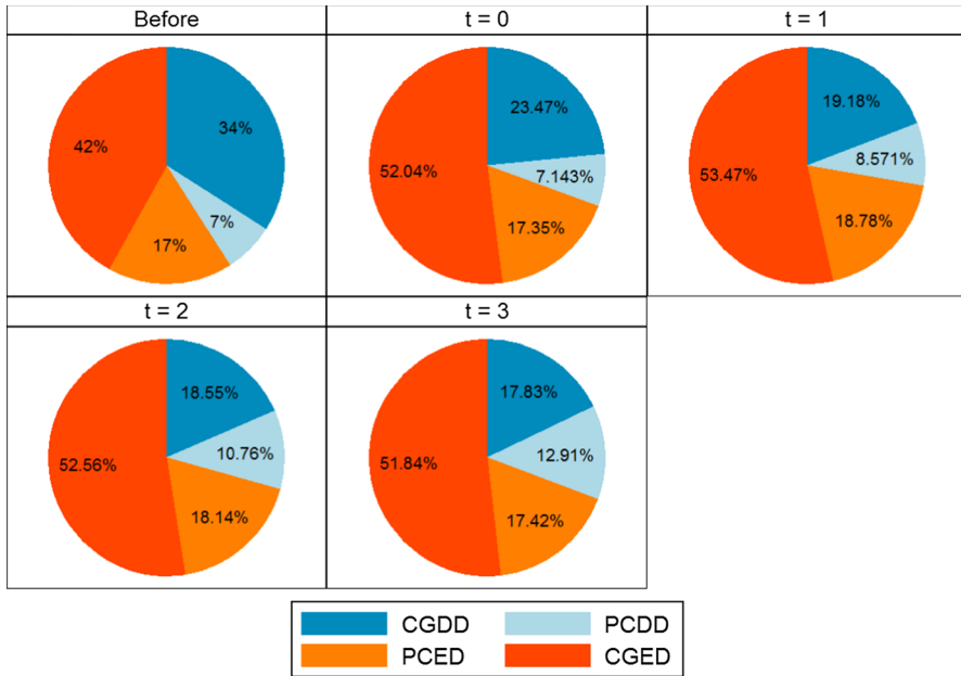
Fig. 3 Debt decomposition after storm
