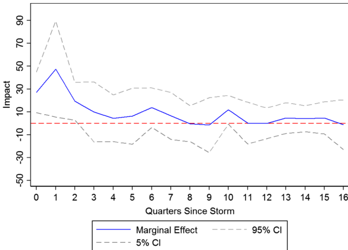
Fig. 2 Long-term impact on debt to GDP ratio
