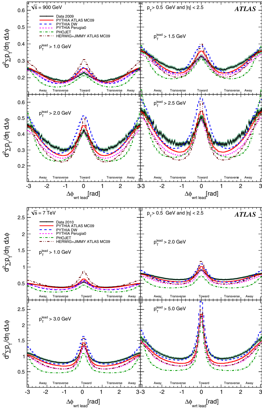
FIG. 9 (color online). ATLAS data at 900 GeV (top plots) and at 7 TeV (bottom plots) corrected back to the particle level, showing the \phi distribution of charged particle p_T densities d^2 p_T/d\eta d\Delta\phi with respect to the leading charged particle (at \Delta\phi = 0 ), for p_T > 0.5 GeV and |\eta| < 2.5 . The leading charged particle is excluded. The data are compared to MC predictions by the PYTHIA ATLAS MC09, DW and Perugia0 tunes, the HERWIG+JIMMY ATLAS MC09 tune, and PHOJET. The distributions obtained by restricting the minimum leading charged particle p_T to different values are shown separately. The plots have been symmetrized by reflecting them about \Delta\phi = 0 . The error bars show the statistical uncertainty while the shaded areas show the combined statistical and systematic uncertainty corresponding to each p_T lower cut value.
