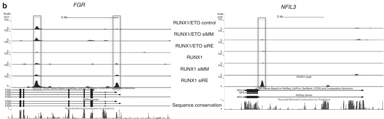
Figure 4. Knockdown of RUNX1/ETO leads to a redistribution of RUNX1 binding. Kasumi-1 cells were electroporated with either mismatch control siRNA (siMM) or RUNX1/ETO siRNA (siRE). Two days after siRNA electroporation, RUNX1 binding was measured by ChIP sequencing in both populations. (a) Top panel: Venn diagram showing the appearance of new RUNX1-binding sites after RUNX1/ETO depletion. Bottom left: Venn diagram showing the overlap between RUNX1/ETO-bound regions and de novo RUNX1 sites, demonstrating that the latter are distinct from sites previously bound by RUNX1/ETO. Bottom right: Venn diagram showing the overlap between RUNX1/ETO-bound sequences and sites bound by RUNX1 before and after RUNX1/ETO depletion. (b) Example of alterations in RUNX1 binding. Left panel shows UCSC browser images depicting one gene ( NFIL3 ) at a site not previously bound by RUNX1/ETO and another gene ( FGR ) showing a de novo RUNX1 with a RUNX1/ETO-bound site showing an increase in RUNX1 binding at this site after knockdown.
