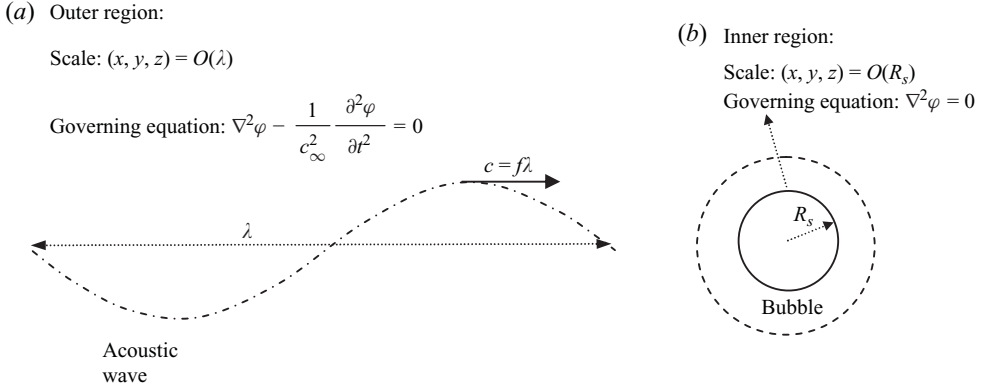
FIGURE 1. A representation of the weakly compressible model for a micro-cavitation bubble subjected to a plane acoustic wave, with speed of sound c_\infty and the wavelength \lambda being much larger than the equilibrium radius of the bubble R_s .
