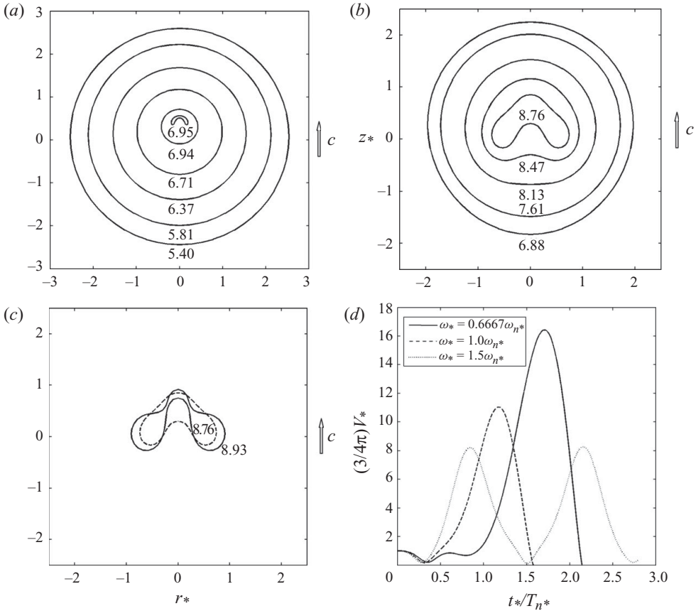
FIGURE 14. Bubble shapes during the third collapse phase for the bubble characterized by (a) b_* = 1.5 , \omega_* = 0.6667\omega_{n*} , (b) b_* = 0.6667 , \omega_* = 1.5\omega_{n*} and (c) for the bubble in (b) during the subsequent rebounding phase. (d) The volume histories of the bubble for the three cases in figures 11(b), 14(a) and 14(b, c).
