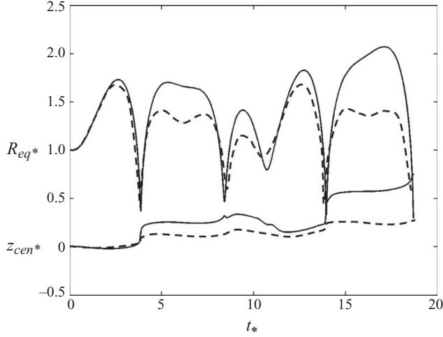
FIGURE 3. The comparison between the MEL (solid line) and the spherical theory (Shaw 2009) (dashed line) for the equivalent radius R_{eq^*} and centroid z_{cen^*} . The parameters for the case are the liquid at p_\infty = 101.3 kPa, \rho_\infty = 998 kg m ^{-3} , c_\infty = 1500 m s ^{-1} ; the bubble at R_0 = 2 \mu m, p_v = 0.023p_\infty , \sigma = 0.0728 N m ^{-1} ; the acoustic wave at f = 1004 kHz, p_a = 1.2(p_\infty - p_v) and \theta_0 = \pi ; \gamma = 1.0 as R \geq R_0 and \gamma = 1.4 as R < R_0 .
