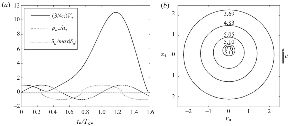
FIGURE 11. (a) Histories of the volume (3/4\pi)V_* , together with the local acoustic pressure p_{a^*}/a_* and the inertial force parameter of the acoustic wave \delta_a/\max|\delta_a| for the bubble characterized by b_* = 1.0 , \omega_* = \omega_{n*} . (b) Bubble shapes during the second collapse phase.
