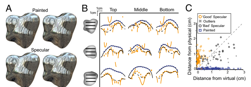
Fig. 6. Example stimuli and results for potato objects. (A) Stereopairs for cross-fusing. (B) Data from the probe adjustment task. Each row is a single shape; columns show three rasters through the object (locations illustrated on gray-scale depictions next to the axes). Black line, physical surface; orange line, virtual surface. Settings are shown for painted (blue squares) and specular (orange circles) conditions. Error bars show SEM across subjects. (C) Relative proximity of settings to the physical and virtual surfaces. Data from the specular surfaces were separated into three groups: “good” vs. “bad” specular were identified using the disparity detectability constraint; “outliers” corresponded to locations that were below the DDC, but were outliers in relation to the surrounding points. Each datum indicates average probe settings for a given location on a given shape for a single observer.
