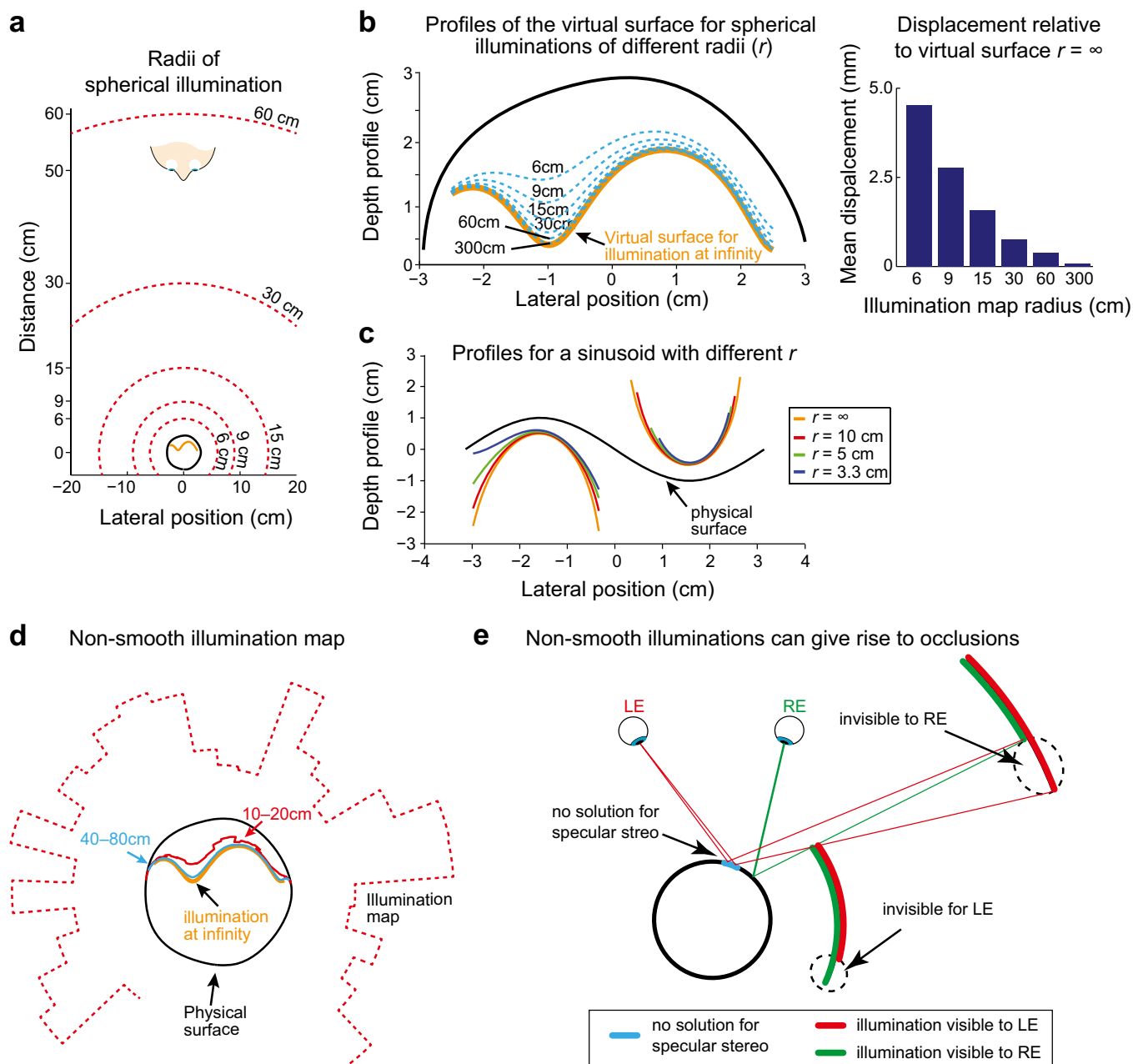
Fig. 55. Effect of illumination distance on the location of the virtual surface. (A) Schematic of the viewing geometry and illumination distances. (B) Virtual surfaces produced by illumination spheres of different radii. Solid orange line shows the profile obtained for illumination at infinity. Virtual surface changes systematically as the illumination gets closer to the object (dotted blue lines). We quantify the difference between the mean depth of the virtual surface at infinity and the other illumination distances (bar graph on Right). (C) Virtual surfaces for a sinusoidal surface that contains both convexities and concavities. (D) Virtual surface under conditions of nonsmooth illumination for a nearby (10–20 cm) and intermediate (40–80 cm) illumination map. (E) Illustration of the potential for occlusion and nonmatchable features arising from specular reflection.
