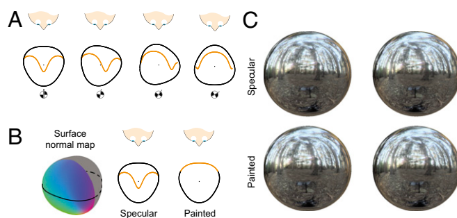
Fig. 2. Properties of the virtual surface and "painted" vs. specular surface rendering. (A) Virtual surface is highly sensitive to both surface and viewing geometry. It can be concave even though the physical surface is convex, and small object rotations lead to large changes in its shape. (B) Near-spherical "muffin" whose surface normals are illustrated using a red-green-blue color representation. Cartoons depict the disparity-defined profile for a slice through the equator of the shape: One for the object rendered with a specular surface, the other for the "painted" case where the illumination map is essentially stuck onto the physical surface. (C) Stereopairs (cross-eyed fusion) for both the painted and specular views of the object from B.
