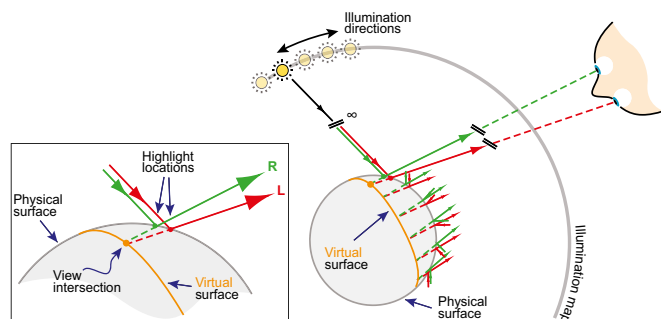
Fig. 1. Physical properties of binocular specular reflections. Reflected features (highlights) appear at different locations in the two eyes' views. Corresponding view rays intersect at locations that are not on the physical surface. Considering light arriving from all different view directions and identifying the matching reflected ray vectors, traces out the "virtual surface."
