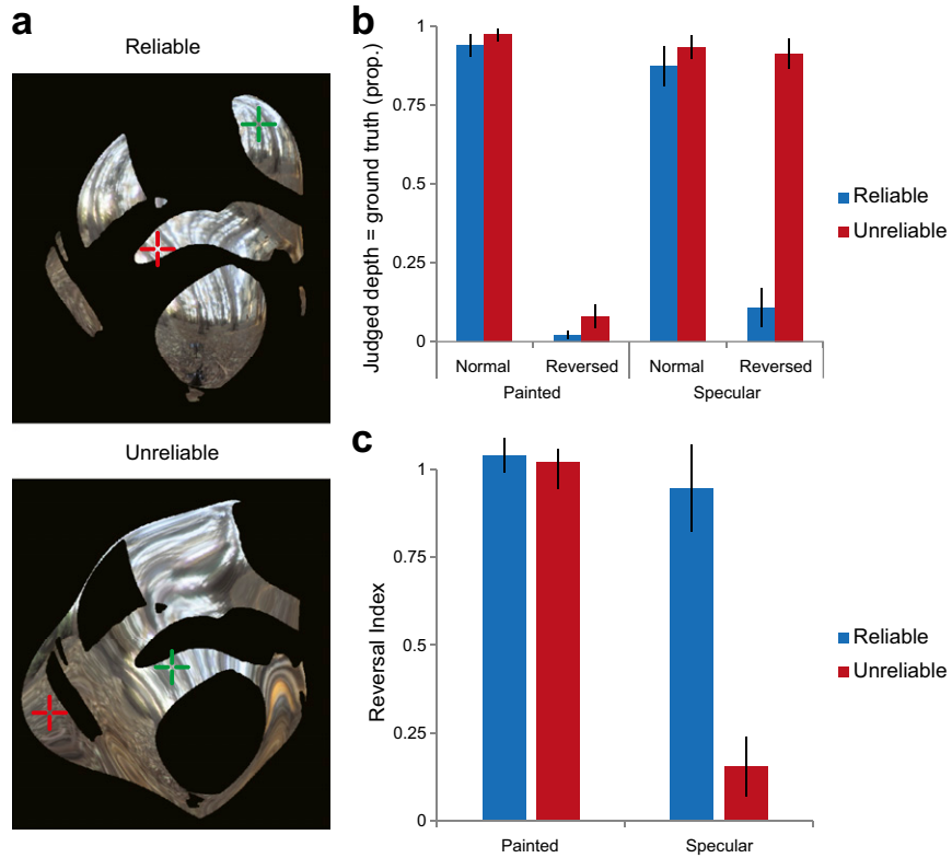
Fig. 54. Experiment in which disparity signals are inverted by swapping the eyes' views. (A) Monocular images of the stimuli (in the experiment the stimuli were presented binocularly). The red/green crosses are shown to illustrate locations at which participants compared the relative depth. (B) Results show proportion judgements that accord to the physical ground truth: a value of 1 means consistent with the physical object and zero consistently opposite the physical object. (C) Data from B expressed as a reversal index ( 2 - (\text{normal} + \text{reversed}) ). Here a value of 1 indicates a full reversal, and zero indicates no reversal.
