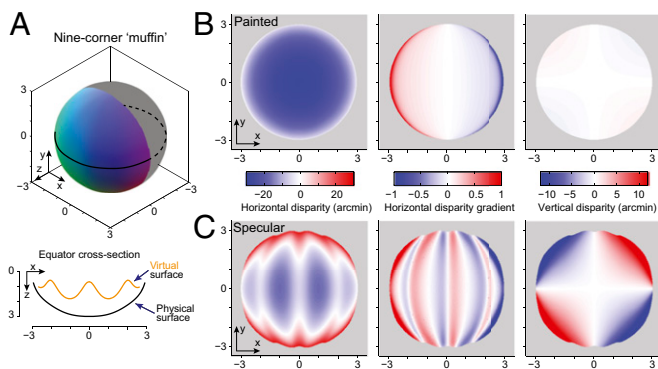
Fig. 3. Example disparity fields of a muffin object. (A) Three-quarters view of a near-spherical nine-cornered muffin (corners are practically invisible). The muffin's surface normals are represented using red-green-blue. A line is projected around the object's equator and the depth profile of the physical and virtual surfaces along this line is shown in cross-section. (B) Maps of horizontal disparity, horizontal disparity gradients, and vertical disparity for a painted nine-cornered muffin. The object is viewed along the depth axis; x , y image locations are in centimeters. The red-blue color code indicates the magnitude of each quantity (color bars are scaled for each column). (C) Pattern of disparities in the virtual manifold produced when viewing the nine-cornered muffin with a specular surface (color scale matched to B).
