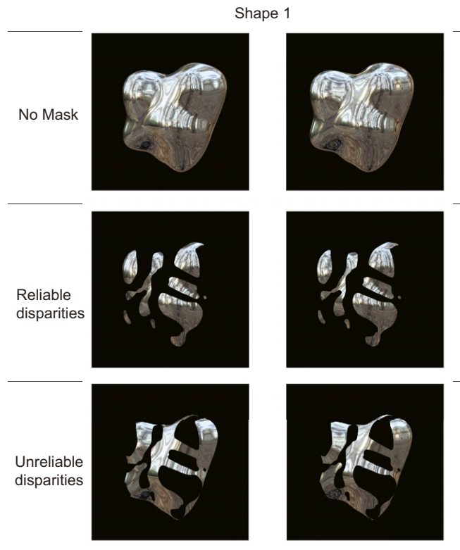
Fig. S3. Isolation of the reliable and unreliable portions of a specular object using a mask. The Top stereopair shows the unmasked object. The Middle stereopair masks off the unreliable parts of the object, so only the more reliable parts (38% of originally visible pixels) are seen. The Bottom row shows the complementary mask, revealing the unreliable parts of the shapes (48% of originally visible pixels). In both cases, the outer contours are masked off (14% of visible pixels).
