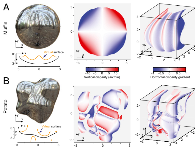
Fig. 4. Illustrations of virtual surface profile of a muffin and potato object. Stimulus examples, the front view, and side view of the virtual surface for a specular muffin (A) and potato (B). Below the stimulus, a depth profile depicts the physical and virtual surfaces as they vary across a horizontal slice through the shape. For the Center and Right columns, the color codes represent vertical disparities ( Center ) and horizontal disparity gradients ( Right ). Note that vertical disparities can be very large for the potato object.
