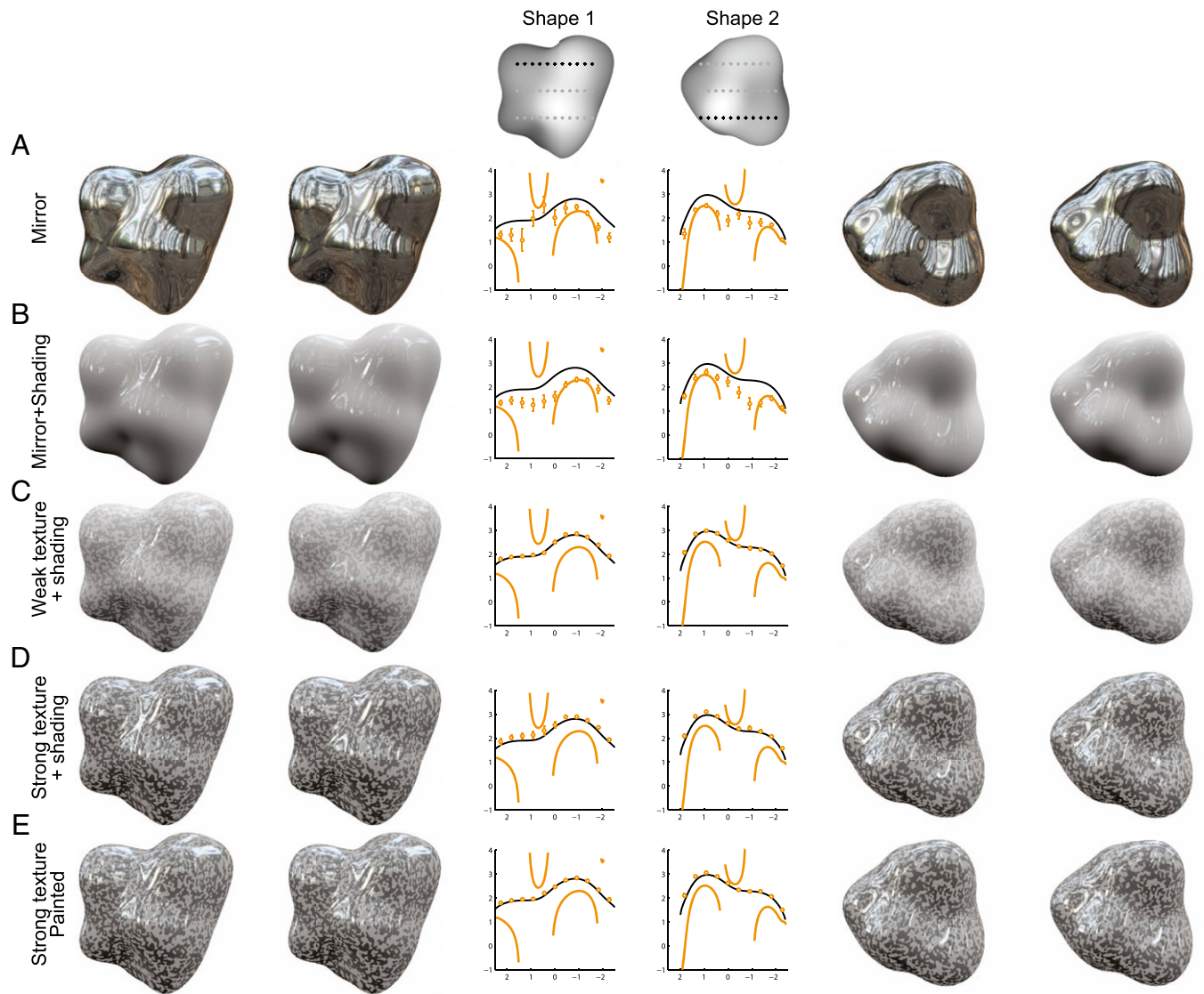
Fig. S2. Stereopairs and results for settings for objects whose surfaces combined specular reflection, shading, and texture. (A) Mirror condition: only specular reflection component is available, participants' settings are close to the virtual surface (similar to Fig. 6). (B) Mirror and shading: specular reflection and shading are combined. (C) Weak texture: specular reflection, shading and low contrast texture components are available. (D) Strong texture, same as C, but texture has stronger contrast. (E) As in D, except that the reflection is attached to the physical surface ("painted" condition).
