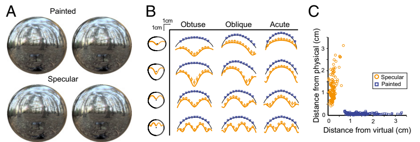
Fig. 5. Example stimuli and results for muffin objects. (A) Stereopairs for cross-fusing. When viewed monocularly, painted and specular stereopairs are almost indistinguishable. When fused, the painted stereopair appears more matte and more spherical. (B) Data from the probe adjustment task. Each row is a single shape viewed at three orientations relative to the viewer. Black line, physical surface; orange line, virtual surface. Settings are shown for painted (blue squares) and specular (orange circles) conditions. Error bars show SEM across observers. (C) Scatterplot of settings in terms of distance from the physical (y axis) and virtual (x axis) surfaces. Each datum represents the mean setting (across repetitions) of an individual observer for a particular location on one of the shapes.
