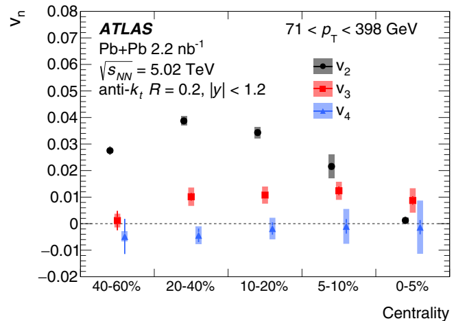
FIG. 8. v_2 , v_3 , and v_4 as a function of centrality for jets with p_T = 71 –398 GeV. The error bars represent the statistical error from the fits, while the error boxes represent the systematic uncertainties.
