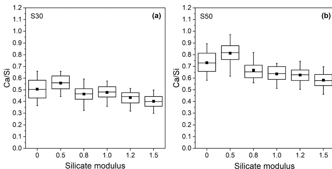
Fig. 8. Box plot of Ca/Si ratio of main reaction products in (a) S30 and (b) S50 AASF pastes. In the box plot, the median value (–), the mean (■), the values at 25% and 75% (box edges), and the values at 5% and 95% level (whiskers) are illustrated.
