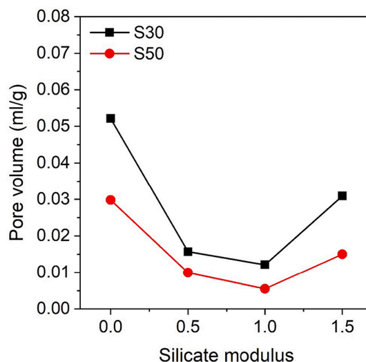
Fig. 12. Capillary porosity ( >0.01 \mu\text{m} ) of AASF pastes at 28 days as a function of activator silicate modulus 0, 0.5, 1.0, and 1.5.
