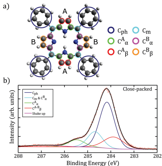
Fig. 2 (a) Assignment of carbon environments within the 2H -TPP molecule based on work by Nardi et al. 21 (b) C1s XP spectra for the close-packed phase of 2H -TPP on Au(111), based upon the assignments in (a), showing a peak structure consistent with previous reports. 21
