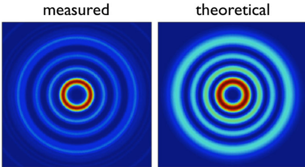
Figure 7. Comparison between the intensity distribution of the composite beam generated by the phase plate (left) and the theoretical intensity distribution for a pure LG 33 beam with same parameters.
