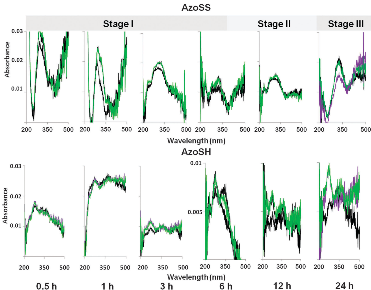
Fig. 7 Typical UV/Vis spectra of AzoSS and AzoSH SAMs at different formation times ( i.e. 0.5 h, 1 h, 3 h, 6 h, 12 h and 24 h) on transparent gold substrates, (---) before and (—) after irradiation at 360 nm for 3 min to switch the molecules in their cis isomer and (—) subsequent irradiation at 480 nm for 3 min to switch in the trans isomer.
