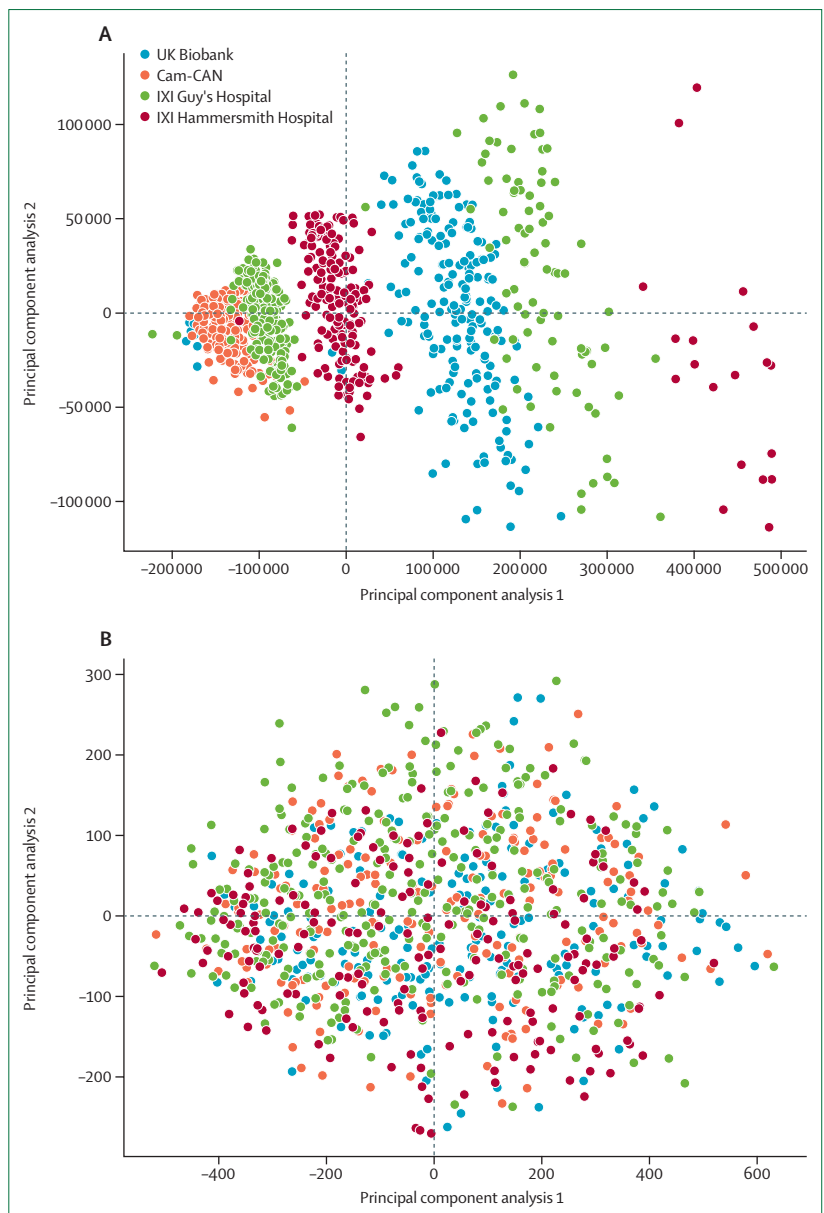
Figure 3: Principal component analysis of brain MRI data, without (A) and with (B) data normalisation, across four hospital sites
