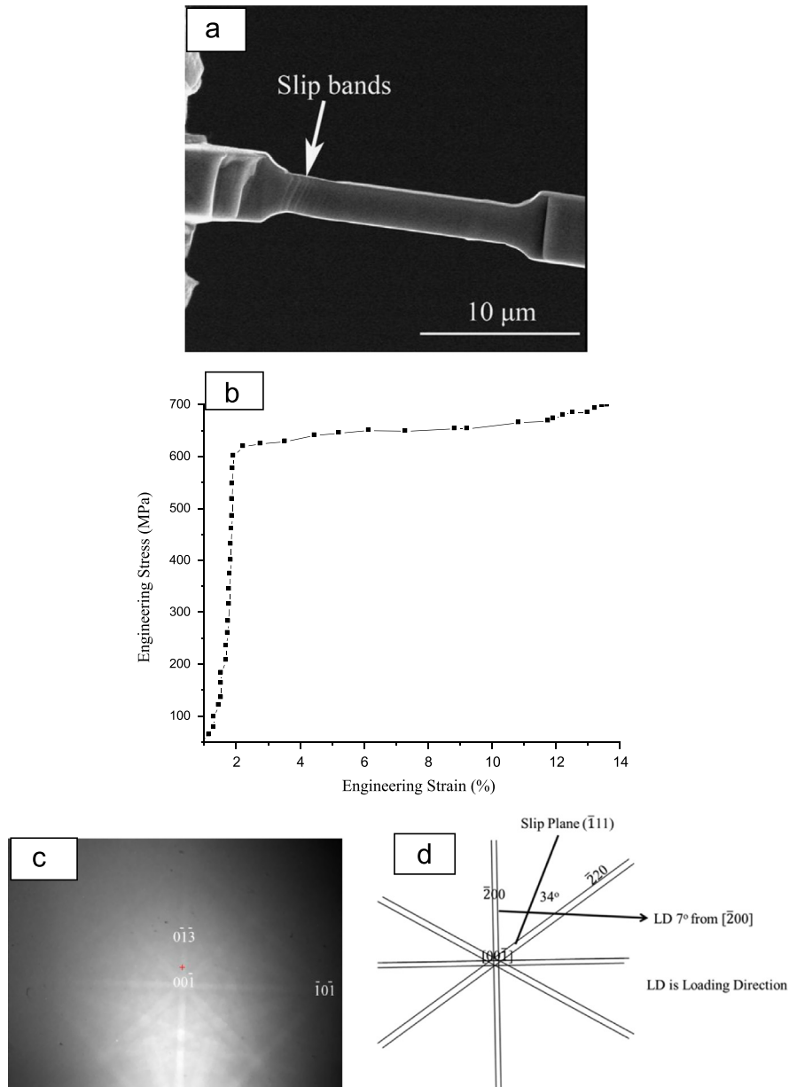
Fig. 3. Micro-tensile sample (a) at 10.8% strain, (b) stress–strain curve of the micro-tensile and (c) EBSD Kikuchi pattern from the specimen with single crystal (foil normal 7° from 00\bar{1} ). Note: All EBSD Kikuchi patterns in this work are analysed with the beam direction pointing downwards. (d) schematic diagram illustrating the orientation relationship between Kikuchi patterns, sample loading direction and slip.
