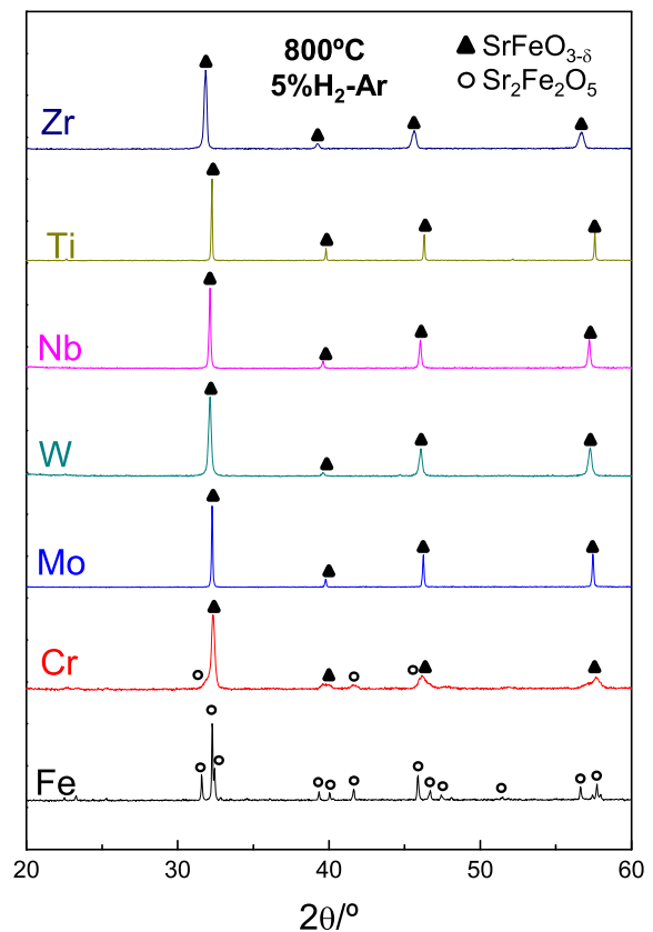
Fig. 3. XRPD patterns for \text{SrFe}_{0.75}\text{M}_{0.25}\text{O}_{3-\delta} ( M = \text{Ti, Zr, Nb, Cr, Mo, W} ) after firing at 800 °C under 5% \text{H}_2\text{-Ar} .
