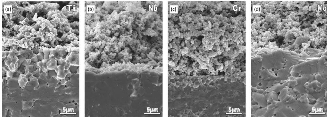
Fig. 8. SEM images of the cross-section of the \text{SrFe}_{0.75}\text{M}_{0.25}\text{O}_{3-\delta} /LSGM interface for a) Ti, b) Nb, c) Cr and d) Mo.
