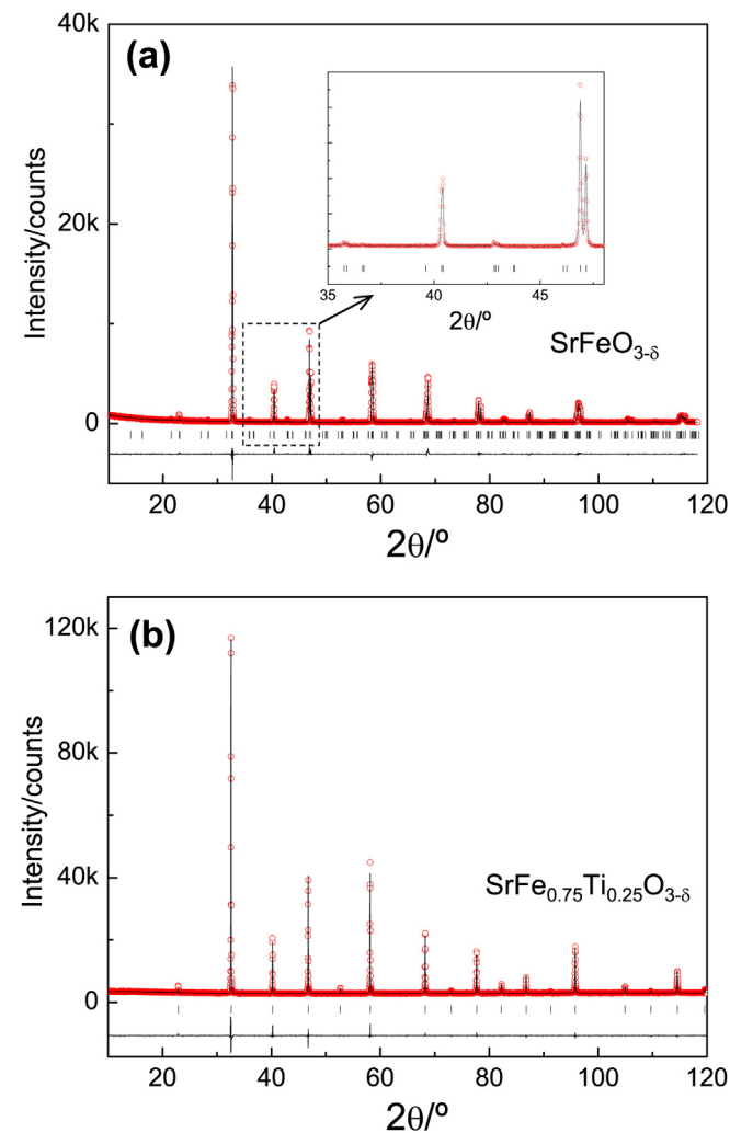
Fig. 2. Rietveld plots [observed data (circles), calculated pattern (full line), and difference curve (bottom)] for (a) orthorhombic (s.g. Cmmm ) \text{SrFeO}_{3-\delta} and (b) cubic (s.g. Pm\text{-}3m ) \text{SrFe}_{0.75}\text{Ti}_{0.25}\text{O}_{3-\delta} .
