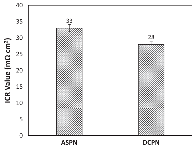
Fig. 10 – ICR value of ASPN and DCPN samples treated under 450^\circ\text{C} , 7 h and 4 mbar.
