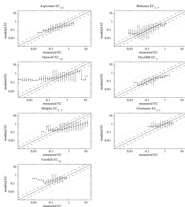
Fig. 4. Scatterplots of measured and modelled EC (standard model setup, STD) for seven European measurement stations: (a) Aspvreten \text{EC}_{10} , (b) Birkenes \text{EC}_{2.5} , (c) Harwell \text{EC}_{10} , (d) Hyttälä \text{EC}_1 , (e) Melpitz \text{EC}_{2.5} , (f) Overtoom \text{EC}_{2.5} , and (g) Vavihill \text{EC}_{10} . The measured EC are divided into logarithmically spaced concentration bins. Each order of magnitude is divided into 10 bins. The points represent the median of the model results for each concentration bin of measured EC. The vertical lines show the range of model results for each bin. Solid lines represent 1 : 1 lines. Dashed lines represent 2 : 1 and 1 : 2 lines, and dotted lines represent 10 : 1 and 1 : 10 lines. Unit: \mu\text{g m}^{-3} .
