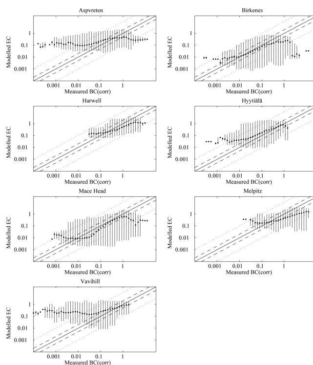
Fig. 7. Scatterplots of hourly measured \text{BC}_e and modelled \text{EC}_{10} (STD model version) for seven European measurement stations: (a) Aspvetren, (b) Birkenes, (c) Harwell, (d) Hyttiälä, (e) Mace Head, (f) Melpitz, and (g) Vavihill. The points represent the median of model results for each concentration bin of measured \text{BC}_e . Each order of magnitude is divided into 10 bins. The vertical lines represent all model results for each bin. Solid lines represent 1 : 1 lines. Dashed lines represent 2 : 1 and 1 : 2 lines and dotted lines represent 10 : 1 and 1 : 10 lines. Unit: \mu\text{g m}^{-3} .
