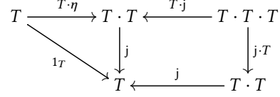
Figure 2. Second and third part of Monad_laws_pointfree
