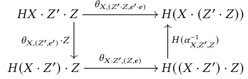
Figure 4. Second strength law for signatures
