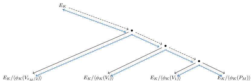
Fig. 3. Naïve attack where isogenies of increasing length need to be recovered. The blue lines represent the meet-in-the-middle computations.
